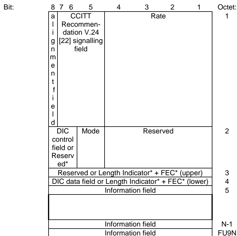
Figure A.1: Frame format type FU9 (an * indicates asynchronous mode only)
