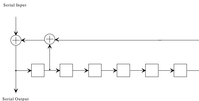
Figure 9: Randomizer
