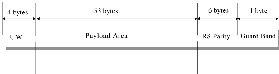
Figure 19: Slot format
