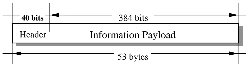
Figure 16: ATM cell format
