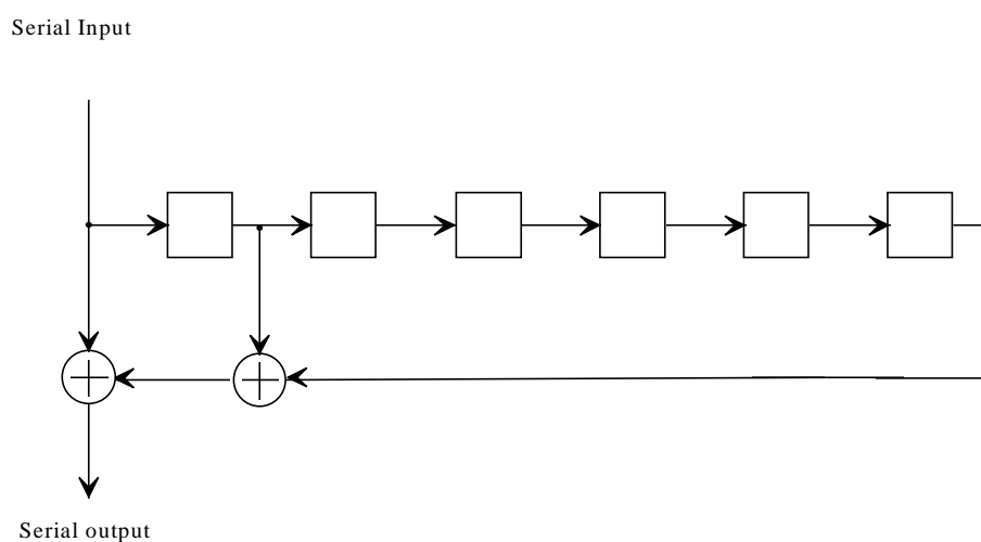
Figure 10: De-randomizer
