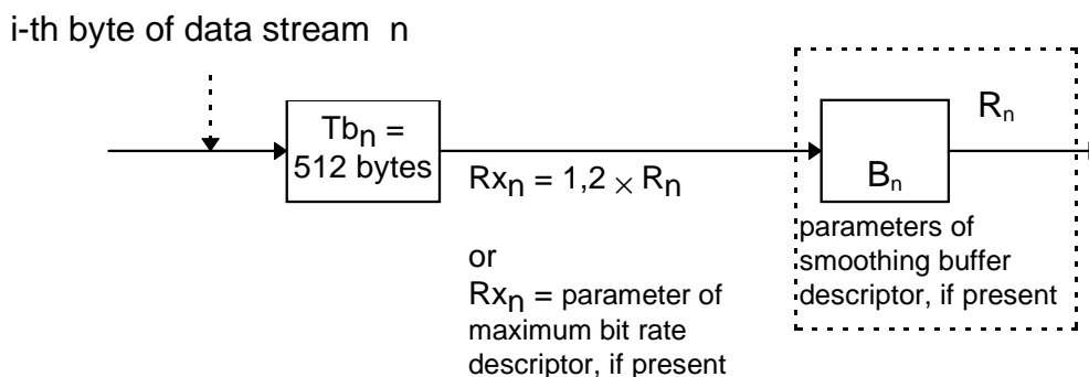
Figure 6: Data service decoder model
