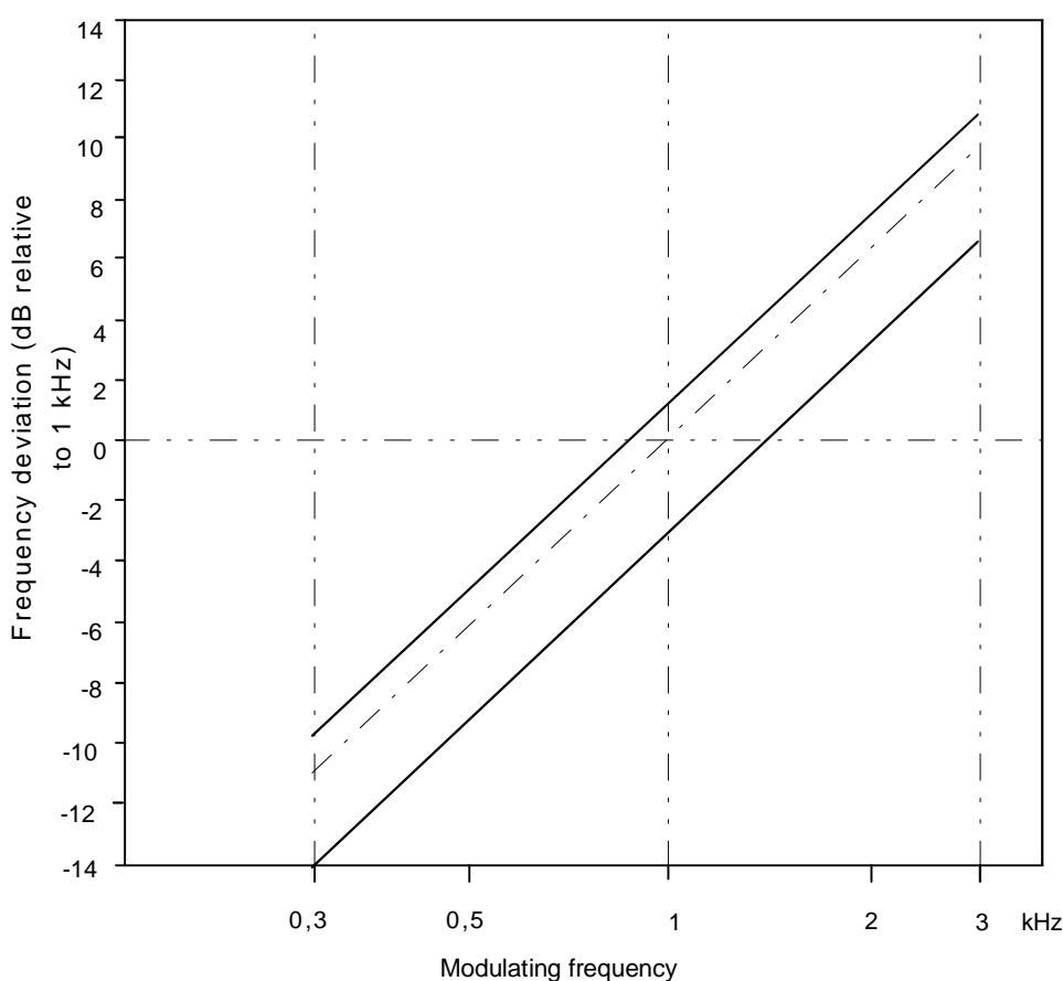
Figure 2: Audio frequency response
