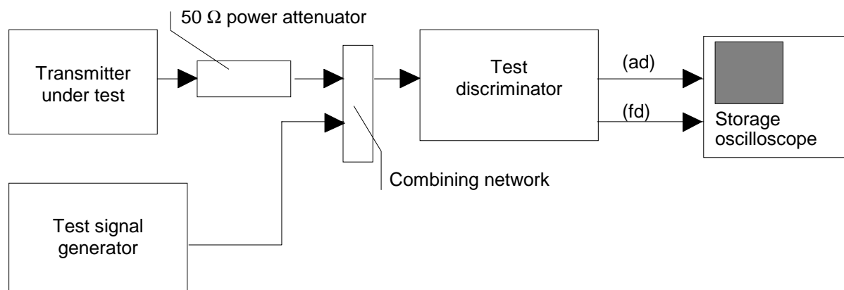
Figure 3: Measurement arrangement
