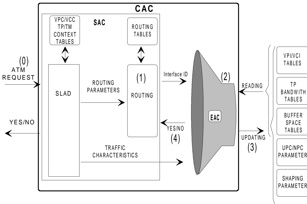
Figure 22: Processing of an ATM request
