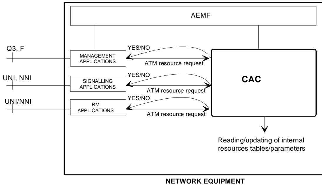
Figure 16: Functions involved for processing an ATM resource request
