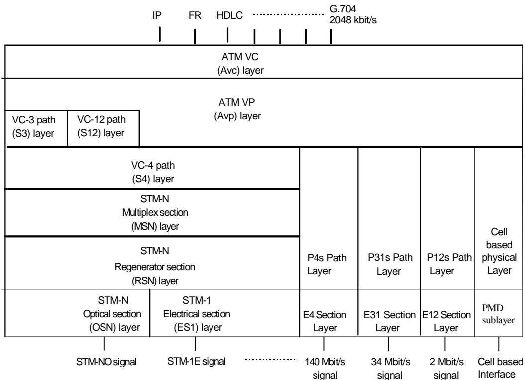
Figure 3: Examples of transmission layers and interface signals
