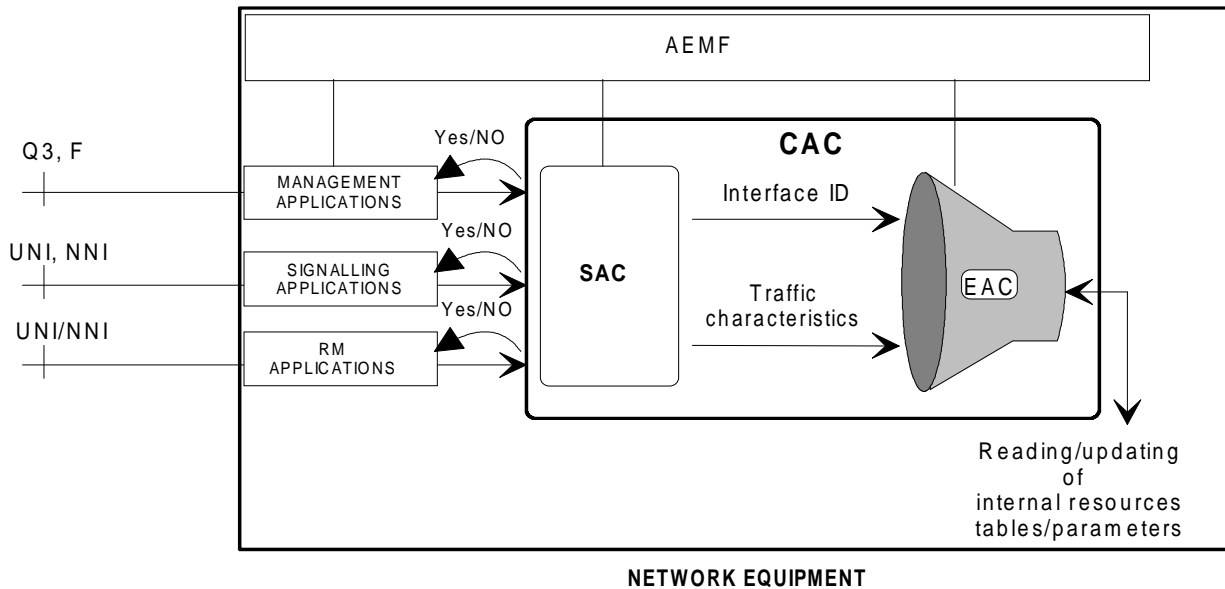
Figure 17: Architecture of the CAC
