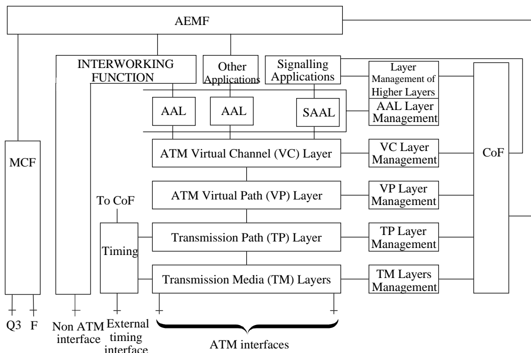
Figure 1: General Overview of ATM Equipment according to ITU-T Recommendation I.731 [30]
