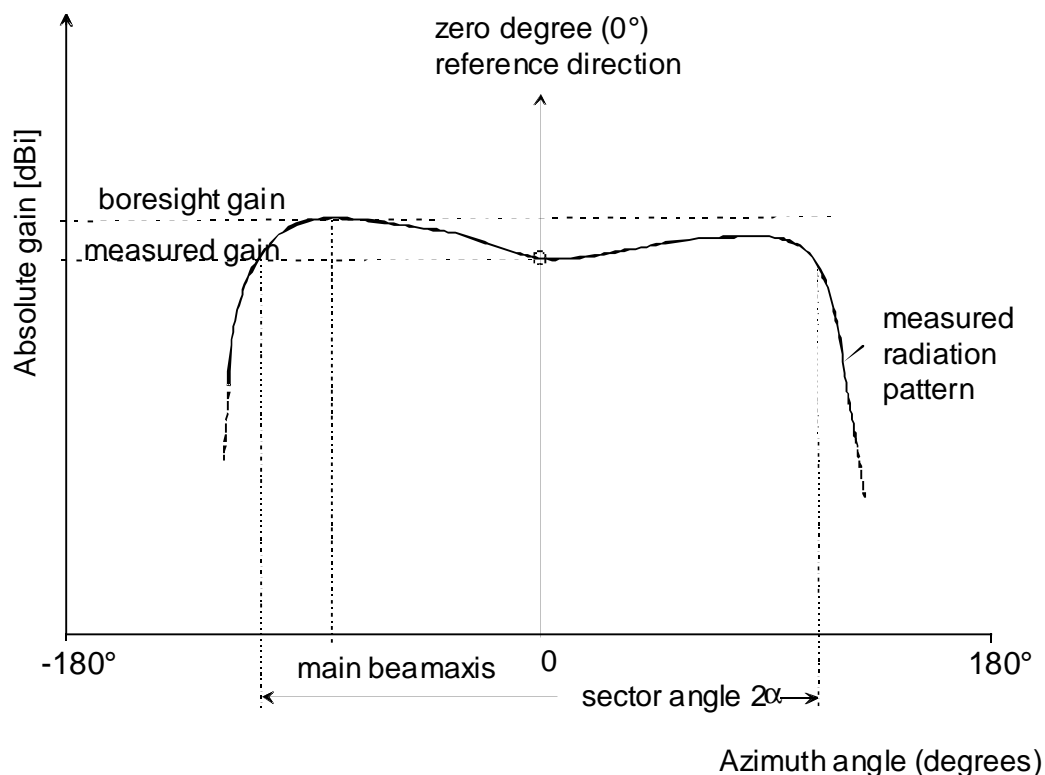
Figure 5: Example of sectored antenna gain measurement
