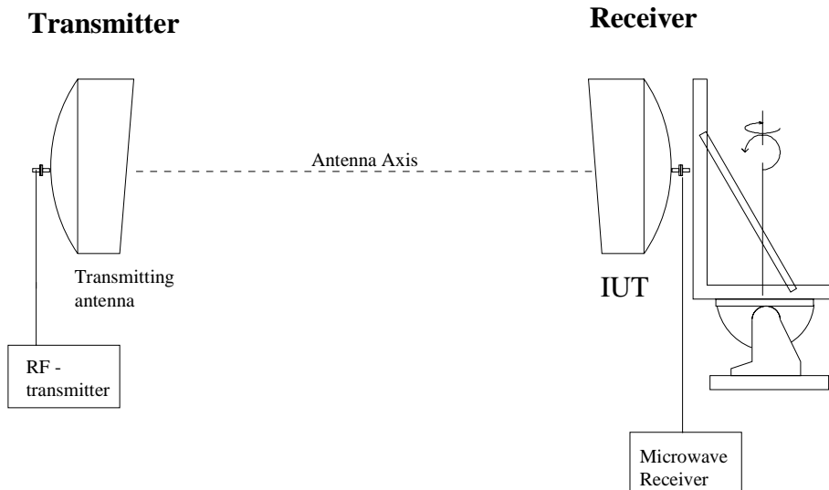
Figure 2: Example of arrangement for the measurement of the radiation pattern
