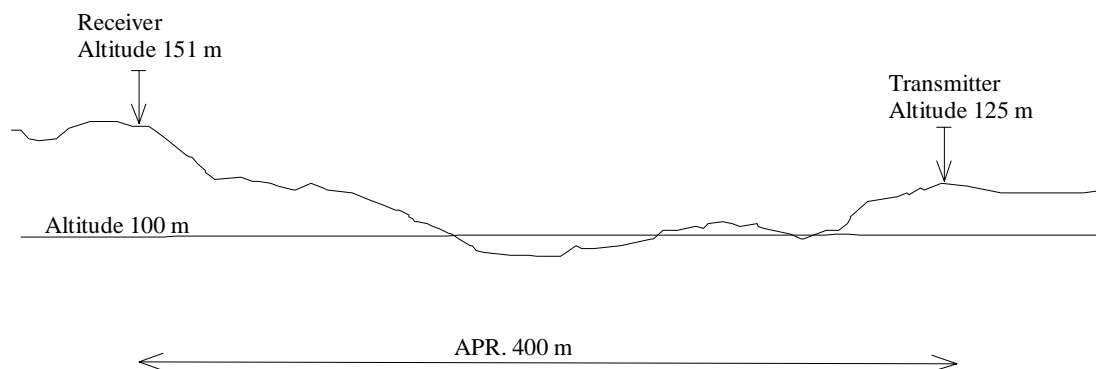
Figure C.1: Terrain profile
