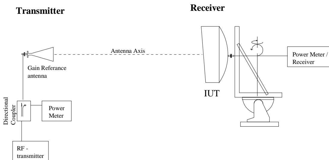
Figure 4b: Test set-up for gain measurement with direct method
