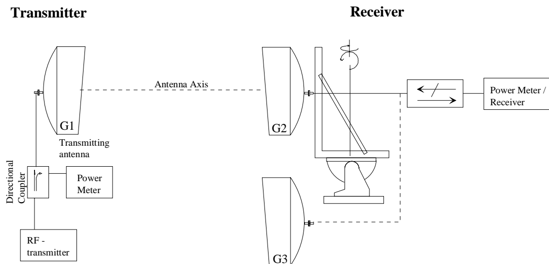
Figure 3b: Test set-up for gain measurement by comparison with a gain reference antenna, using waveguides
