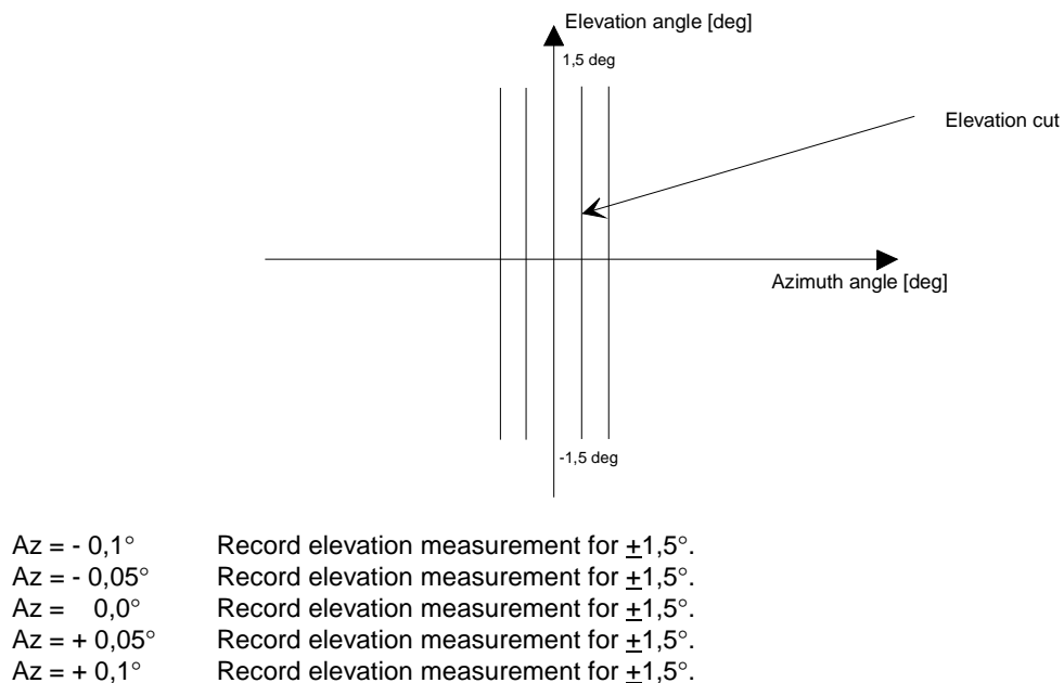
Figure 6: Measurement of the antenna XPD in the region A and additional rectangular part of figure 5
