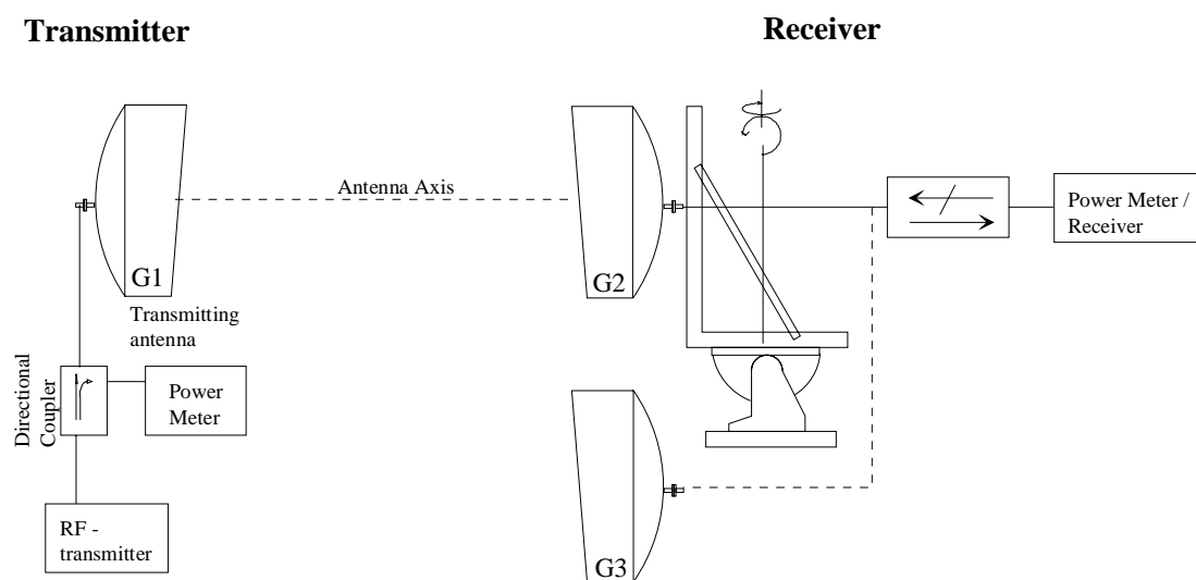
Figure 8a: Test set-up for gain measurement with three antenna method
