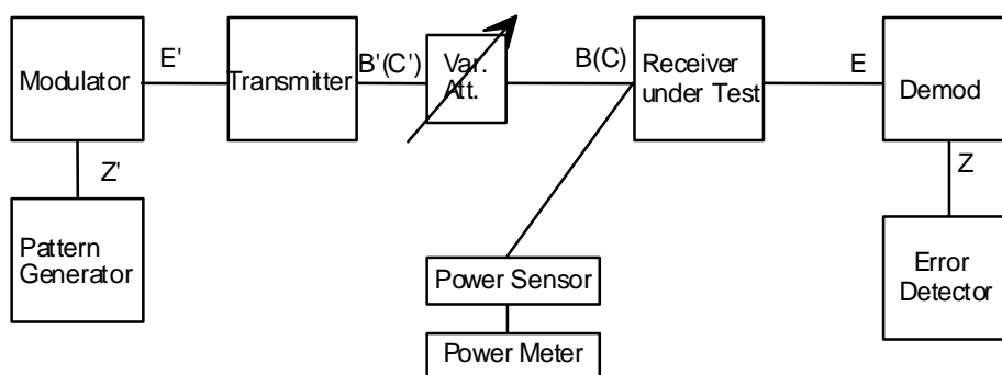
Figure 9: Test configuration for input level range
