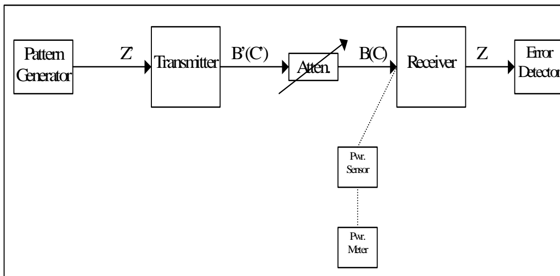
Figure 11: Test configuration for BER as a function of RSL
