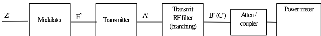
Figure 5: Test configuration for maximum RF output power
