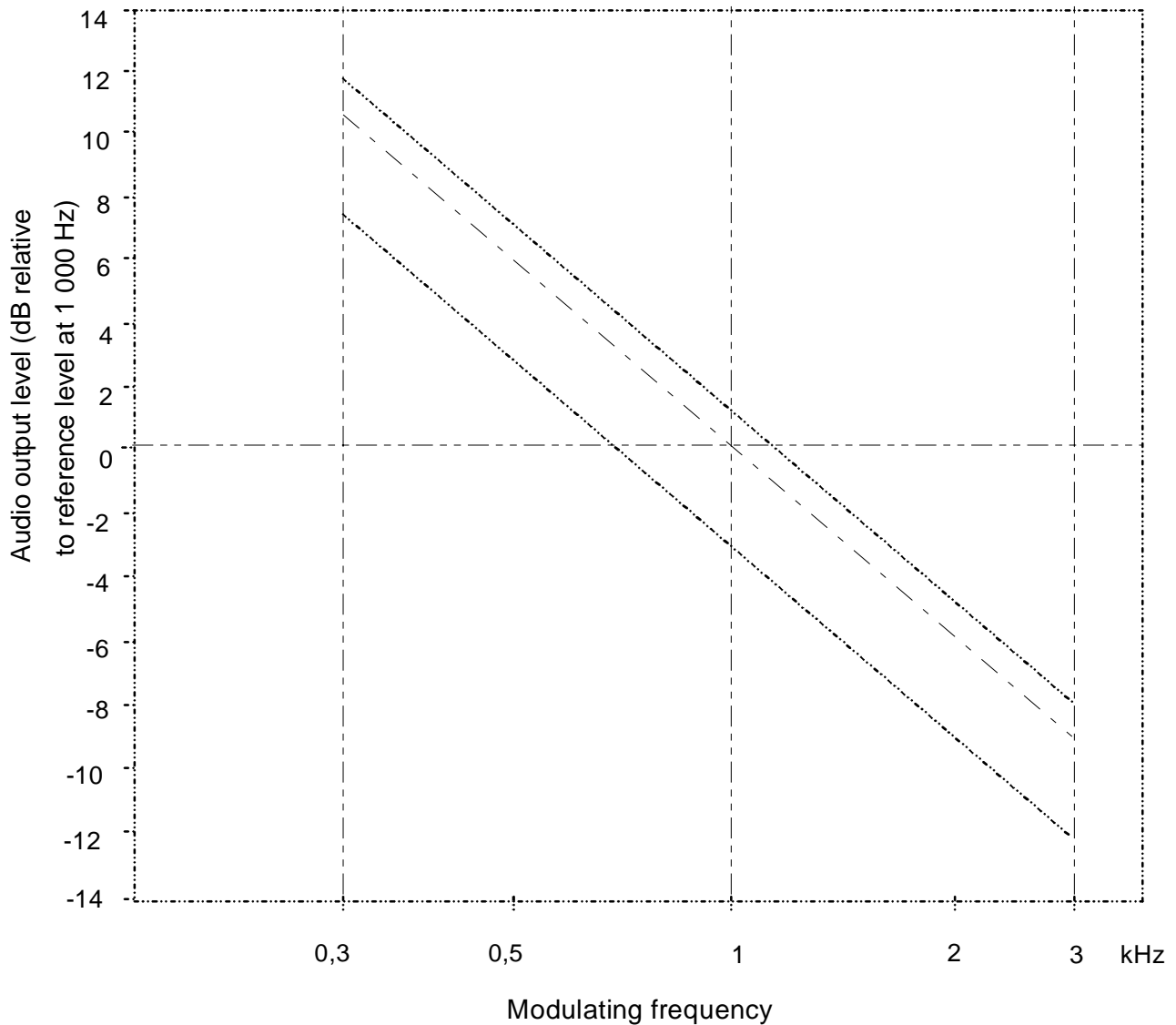
Figure 3: Audio frequency response
