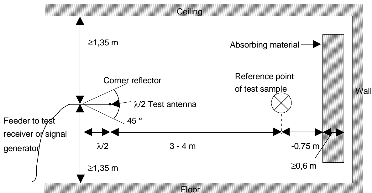
Figure C.2: Indoor site arrangement (shown for horizontal polarization)
