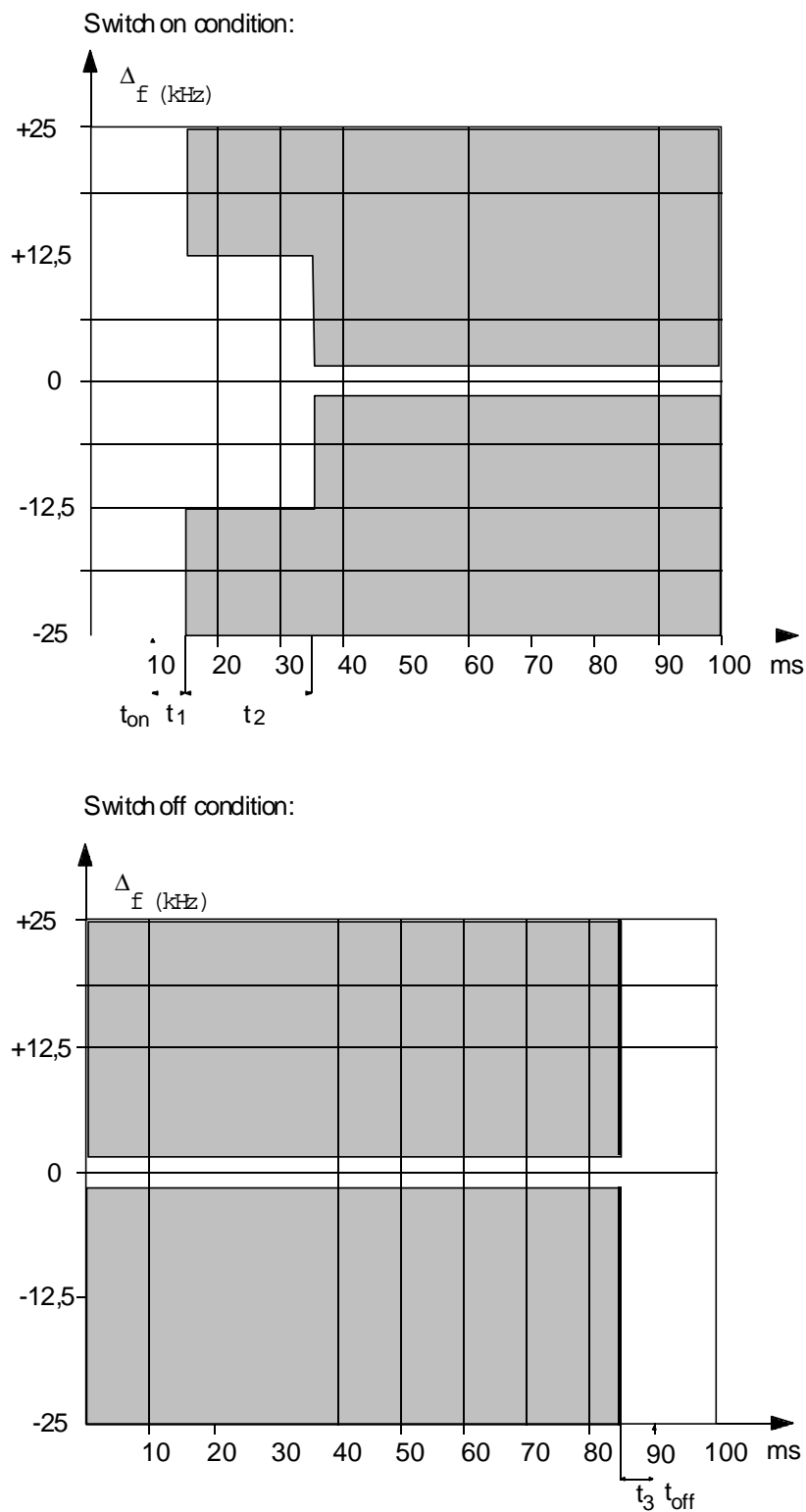
Figure 4: Storage oscilloscope view t_1 , t_2 and t_3
