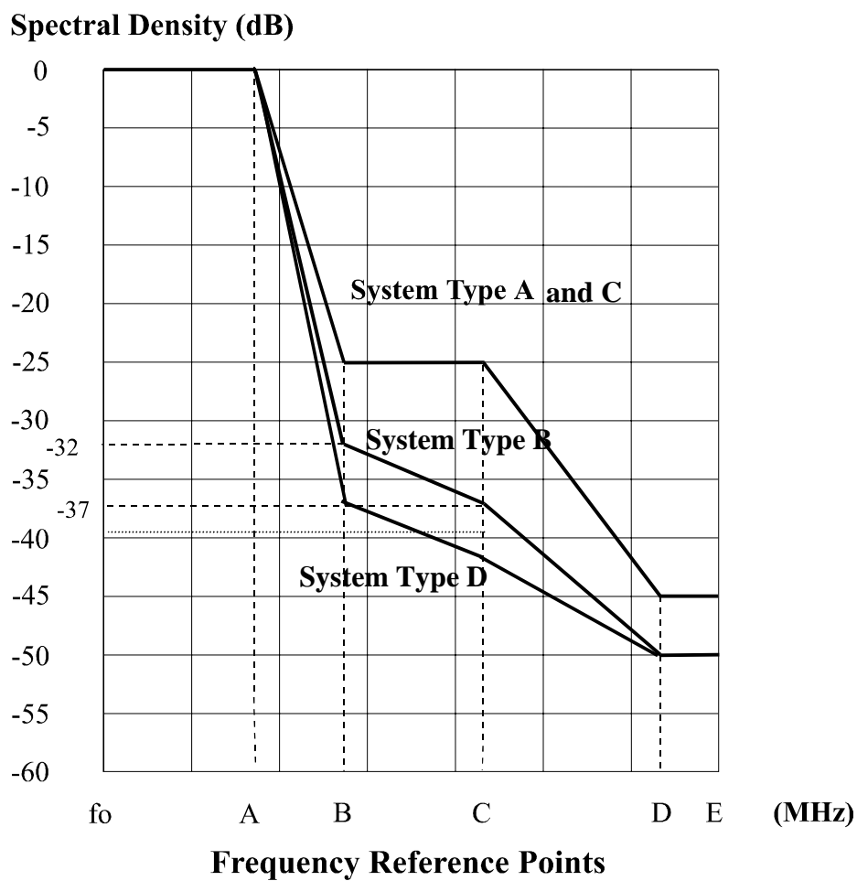
Figure 3: Power spectrum masks (fo = actual carrier frequency)
