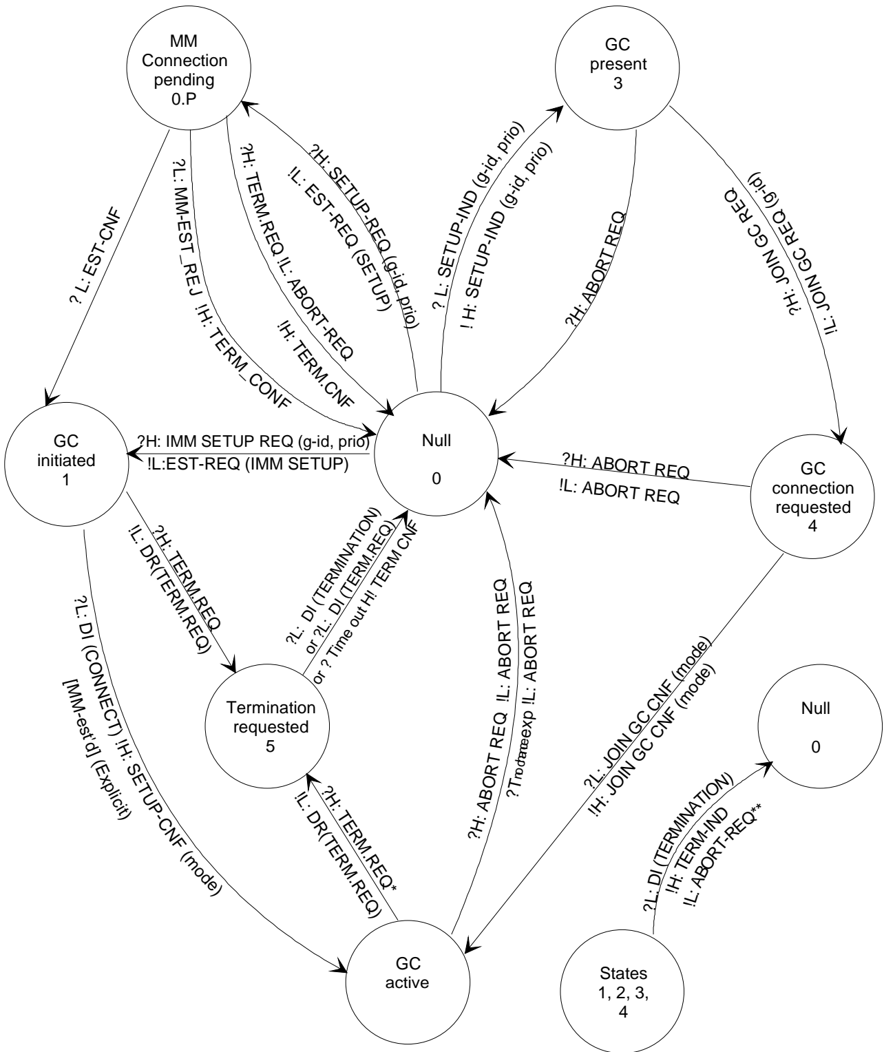
Figure 6.1: Overview group call control protocol/MS side
