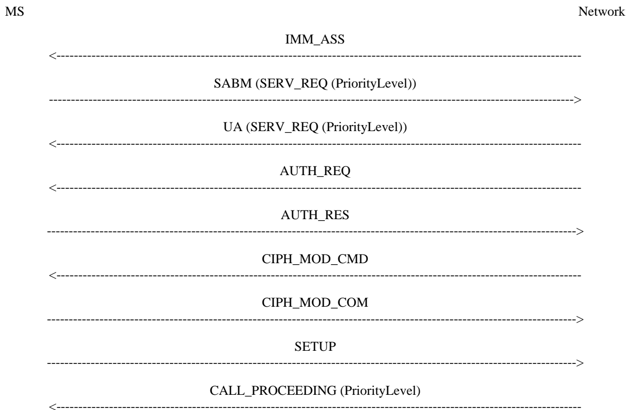
Figure 1: Signalling information required for the prioritisation at mobile originating call establishment
