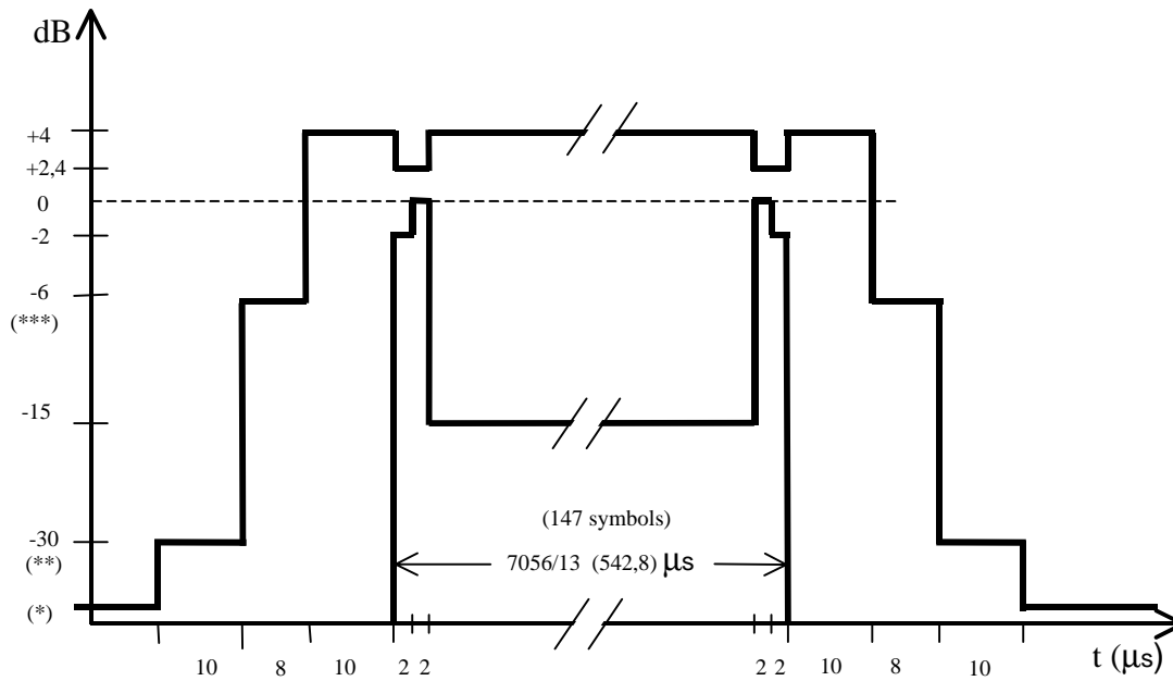
PCS 1900 MS Normal Burst time Mask at 8-PSK modulation
