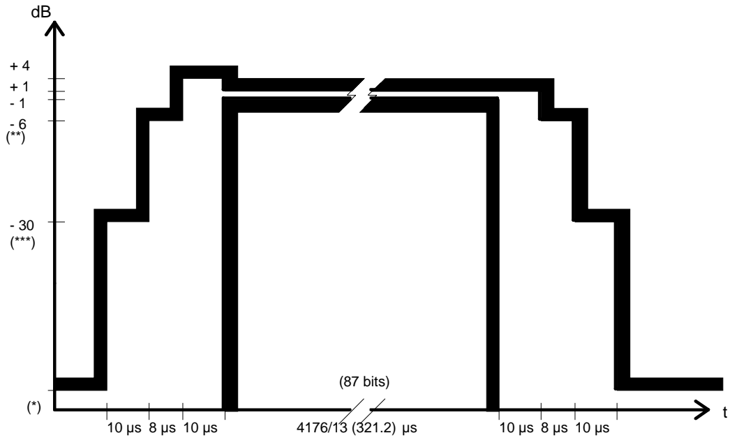
Time mask for access bursts (AB)
