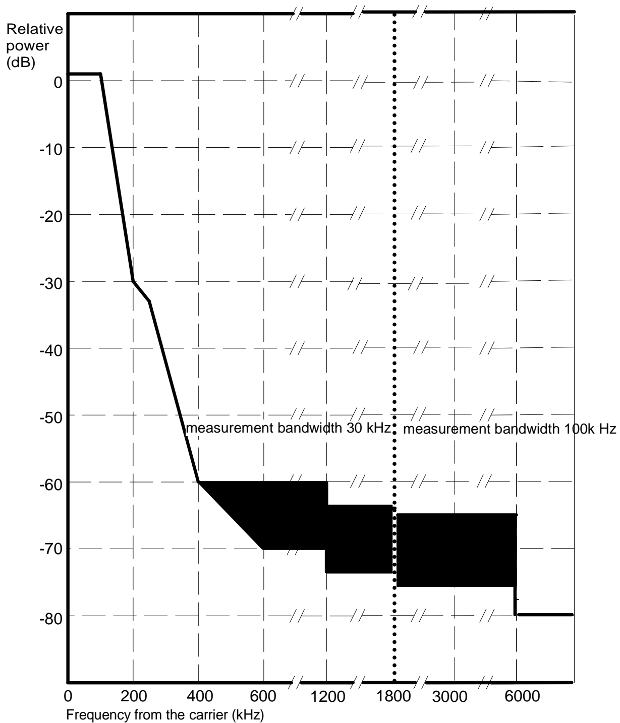
Figure A.2a: GSM 400, GSM 900, GSM 850 and MXM 850 BTS spectrum due to GMSK modulation
