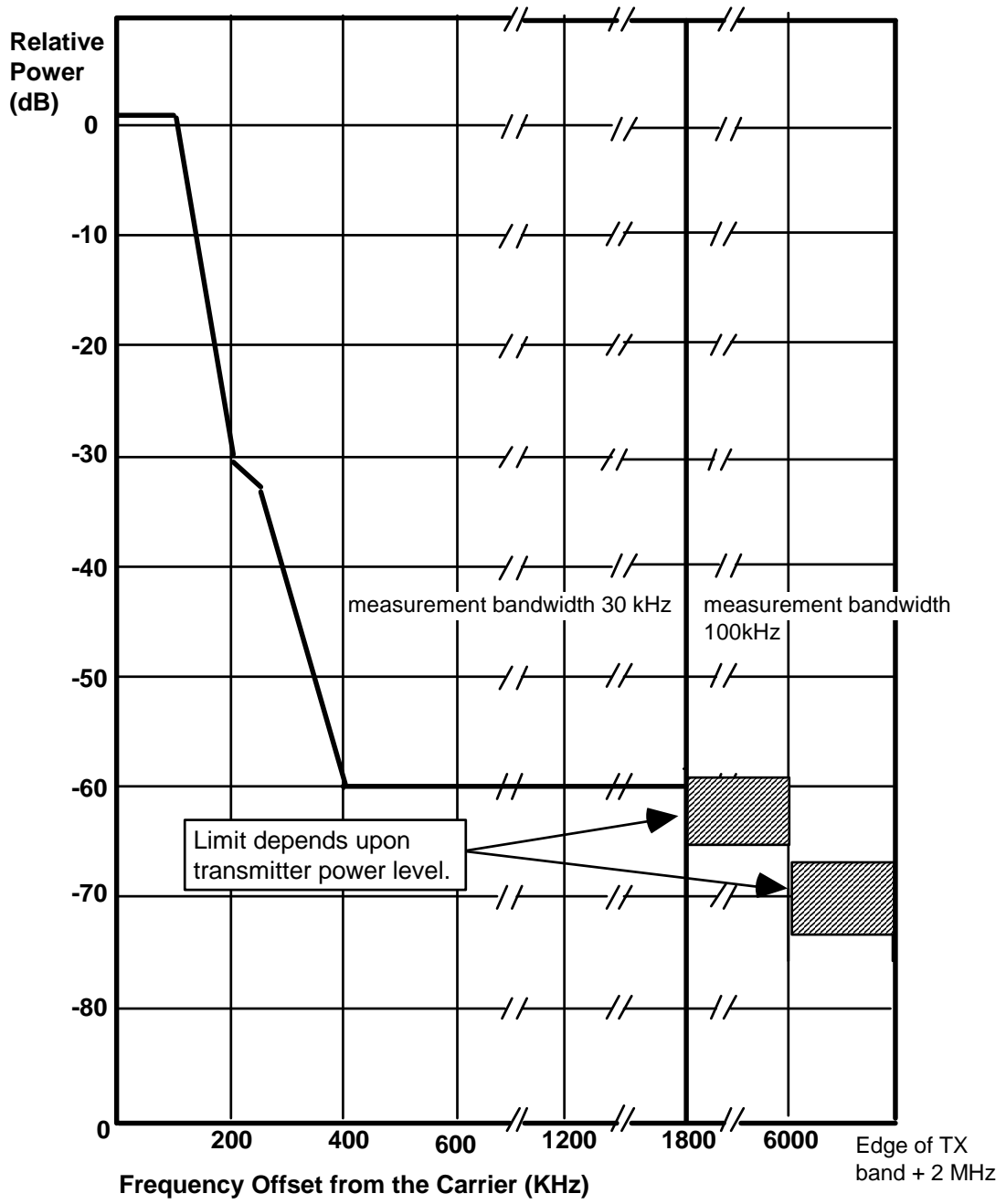
Figure A.5a: PCS 1 900 MS Modulation & Noise Spectrum Mask due to GMSK modulation
