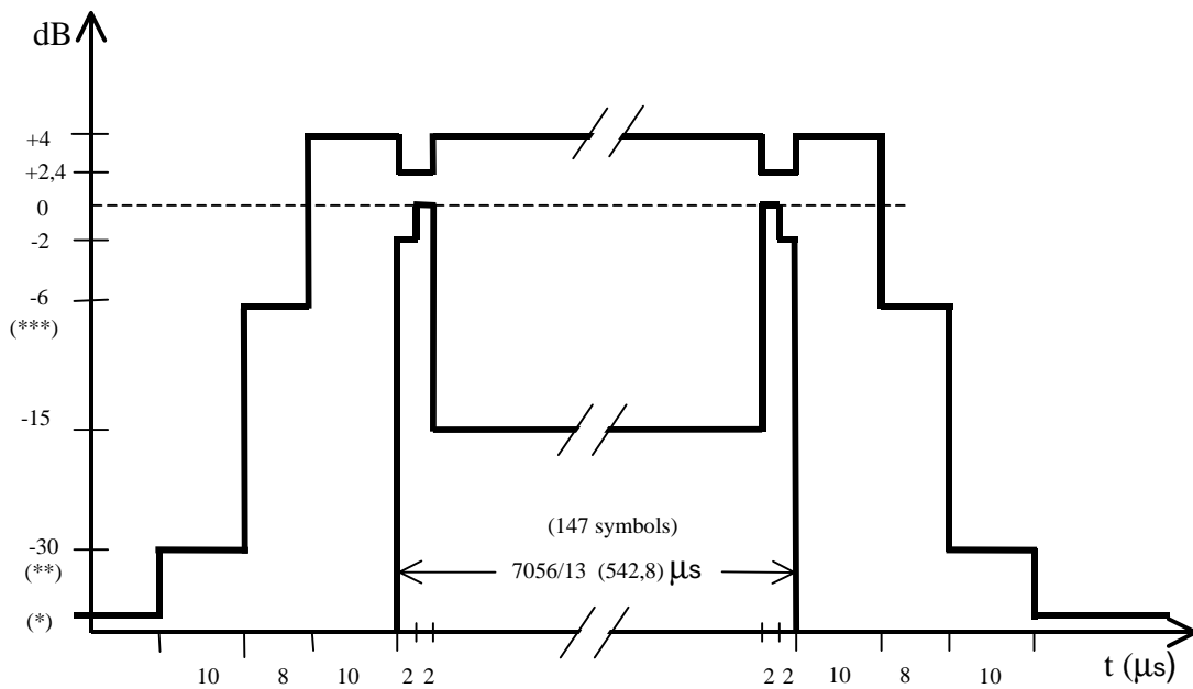
Time mask for normal duration bursts (NB) at 8-PSK modulation
