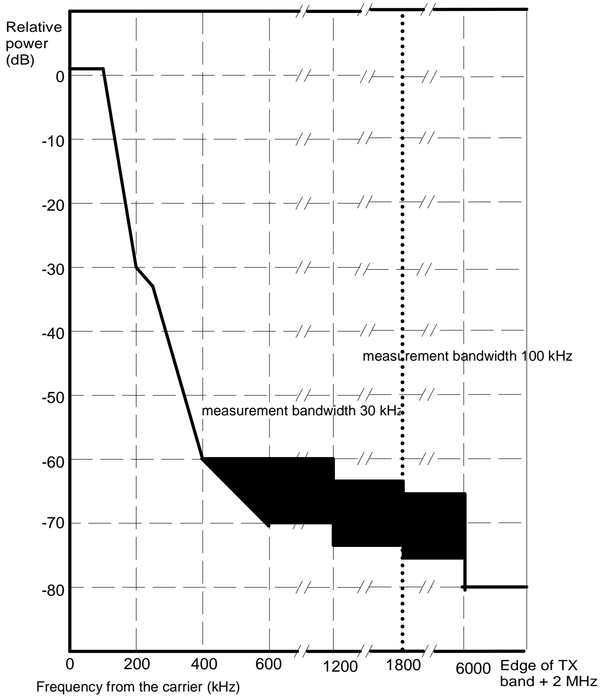
Figure A.4a: DCS 1 800 BTS spectrum due to GMSK modulation
