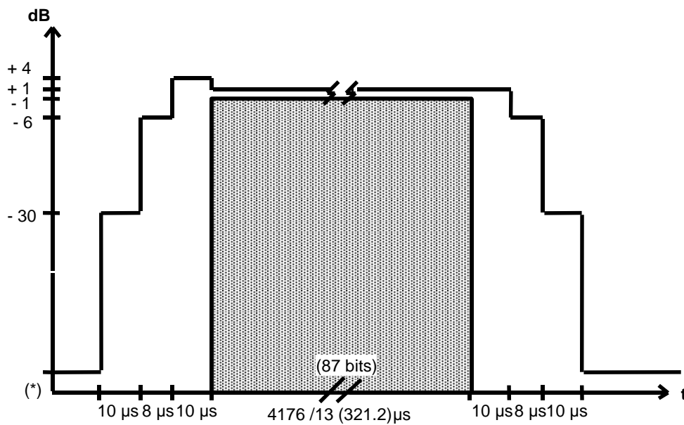
PCS 1900 MS Normal Burst time Mask at 8-PSK modulation
