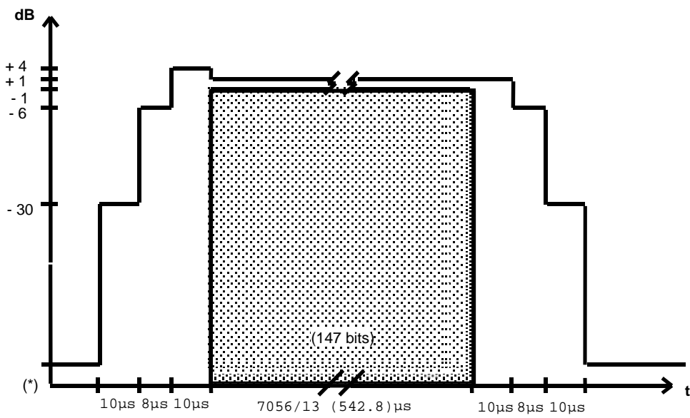
PCS 1900 BTS and MXM 1900 BTS Transmitter Time Mask for normal burst (NB) at 8-PSK modulation
