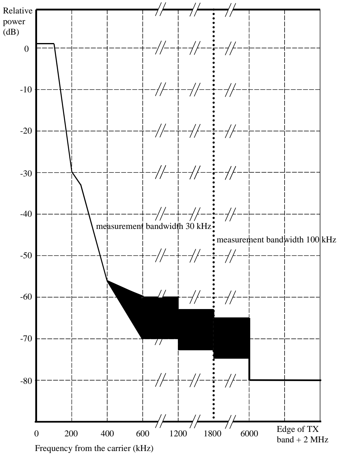
Figure A.2b: GSM 400, GSM 900, GSM 850 and MXM 850 BTS spectrum due to 8-PSK modulation
