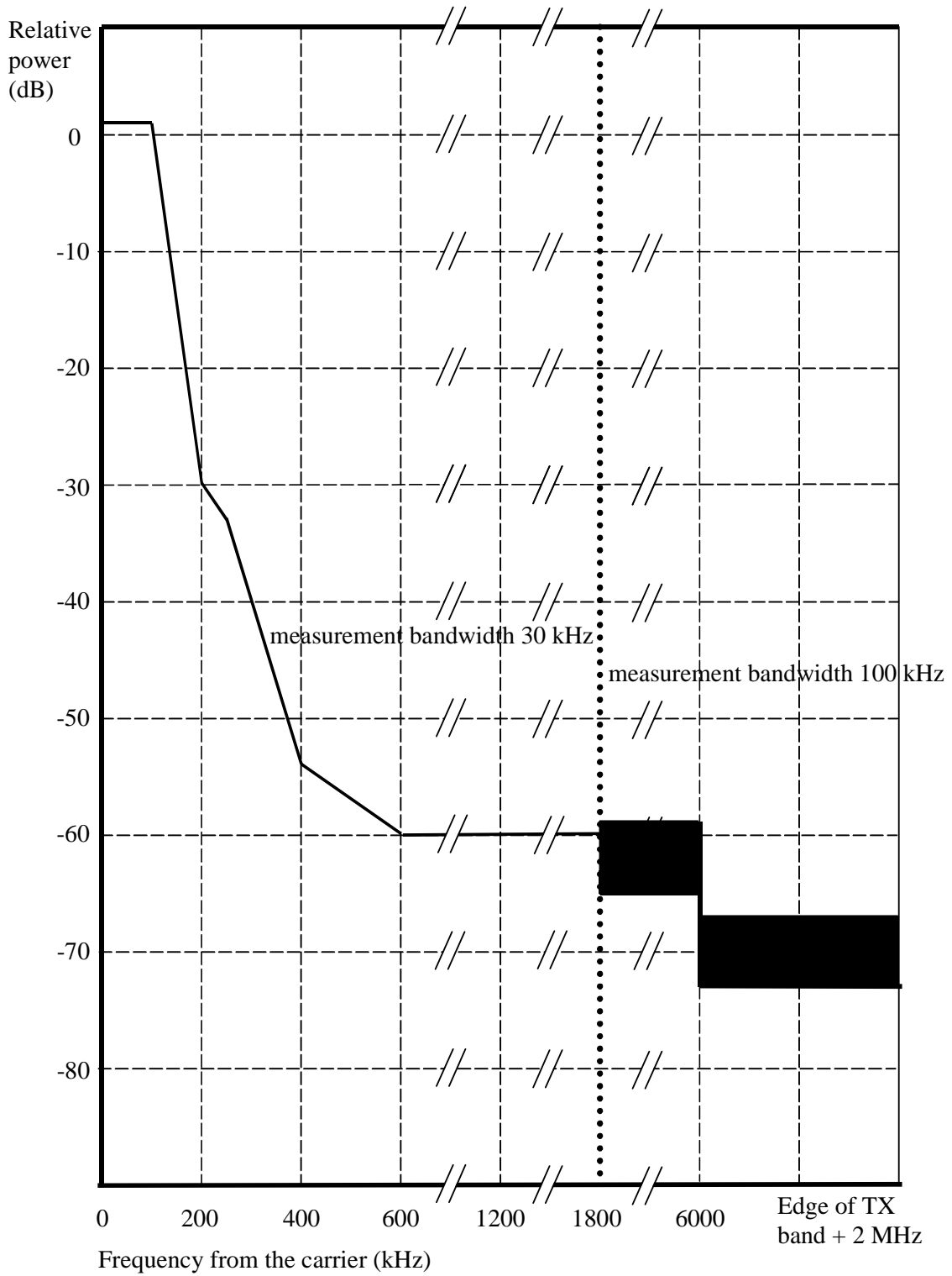
Figure A.3b: DCS 1 800 MS spectrum due to 8-PSK modulation
