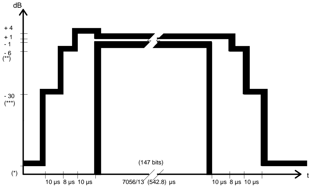
Time mask for normal duration bursts (NB, FB, dB and SB) at GMSK modulation
