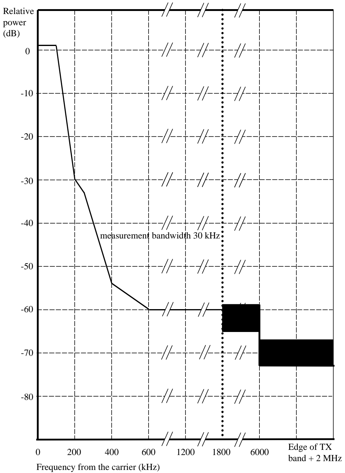
Figure A.5b PCS 1900 MS Modulation & Noise Spectrum Mask due to 8-PSK modulation
