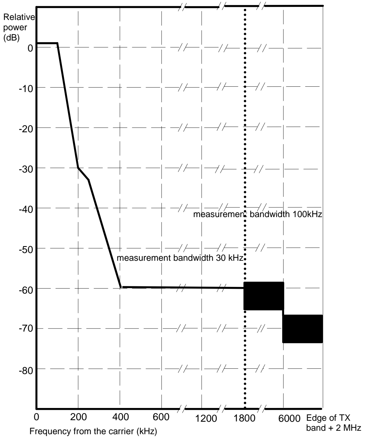
Figure A.3a: DCS 1 800 MS spectrum due to GMSK modulation
