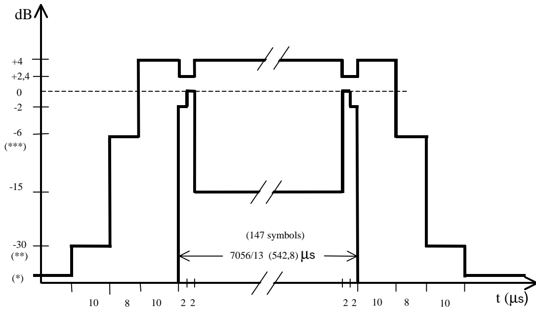
PCS 1900 BTS and MXM 1900 BTS Transmitter Time Mask for normal burst (NB) at 8-PSK modulation
