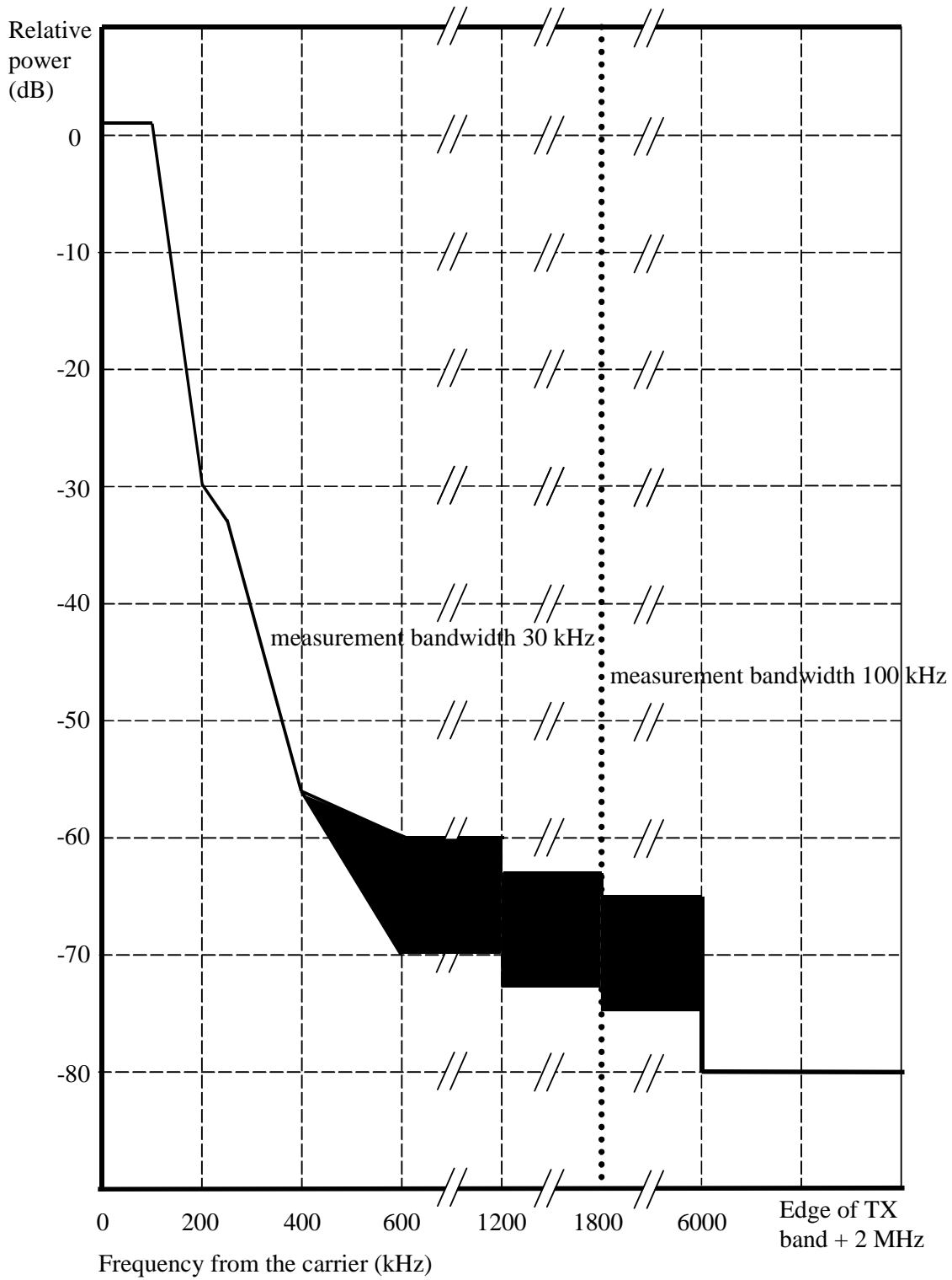
Figure A.4b: DCS 1 800 BTS spectrum due to 8-PSK modulation
