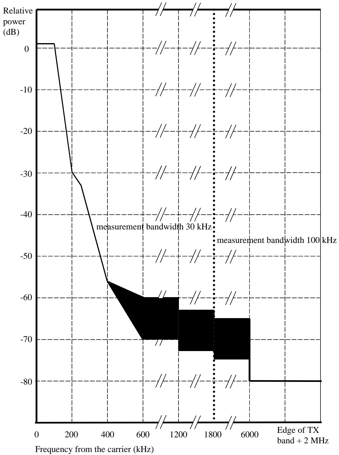
Figure A.6b: PCS 1 900 and MXM 1900 BTS Modulation & Noise Spectrum Mask due to 8-PSK modulation
