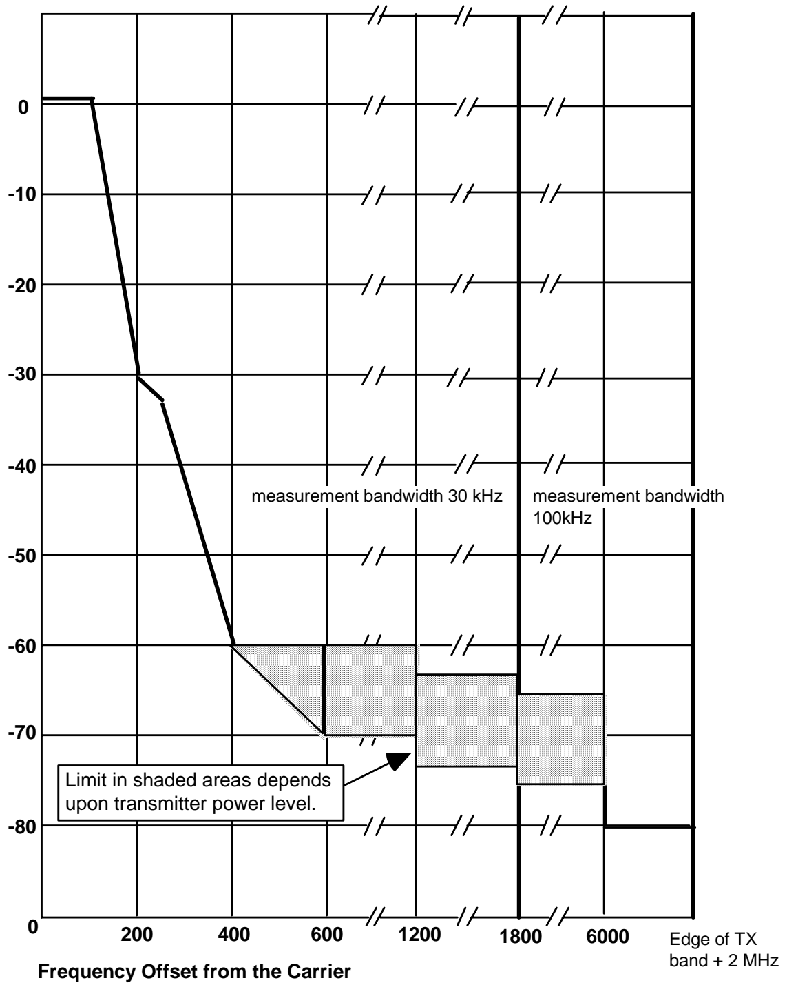
Figure A.6a: PCS 1 900 and MXM 1900 BTS Modulation & Noise Spectrum Mask due to GMSK modulation
