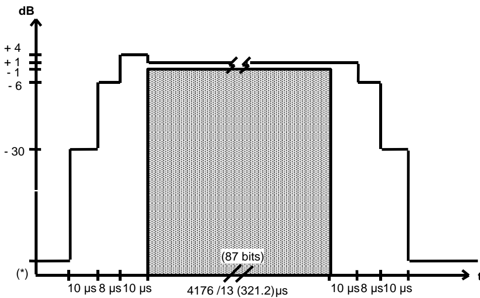
PCS 1900 MS Normal Burst time Mask at 8-PSK modulation
