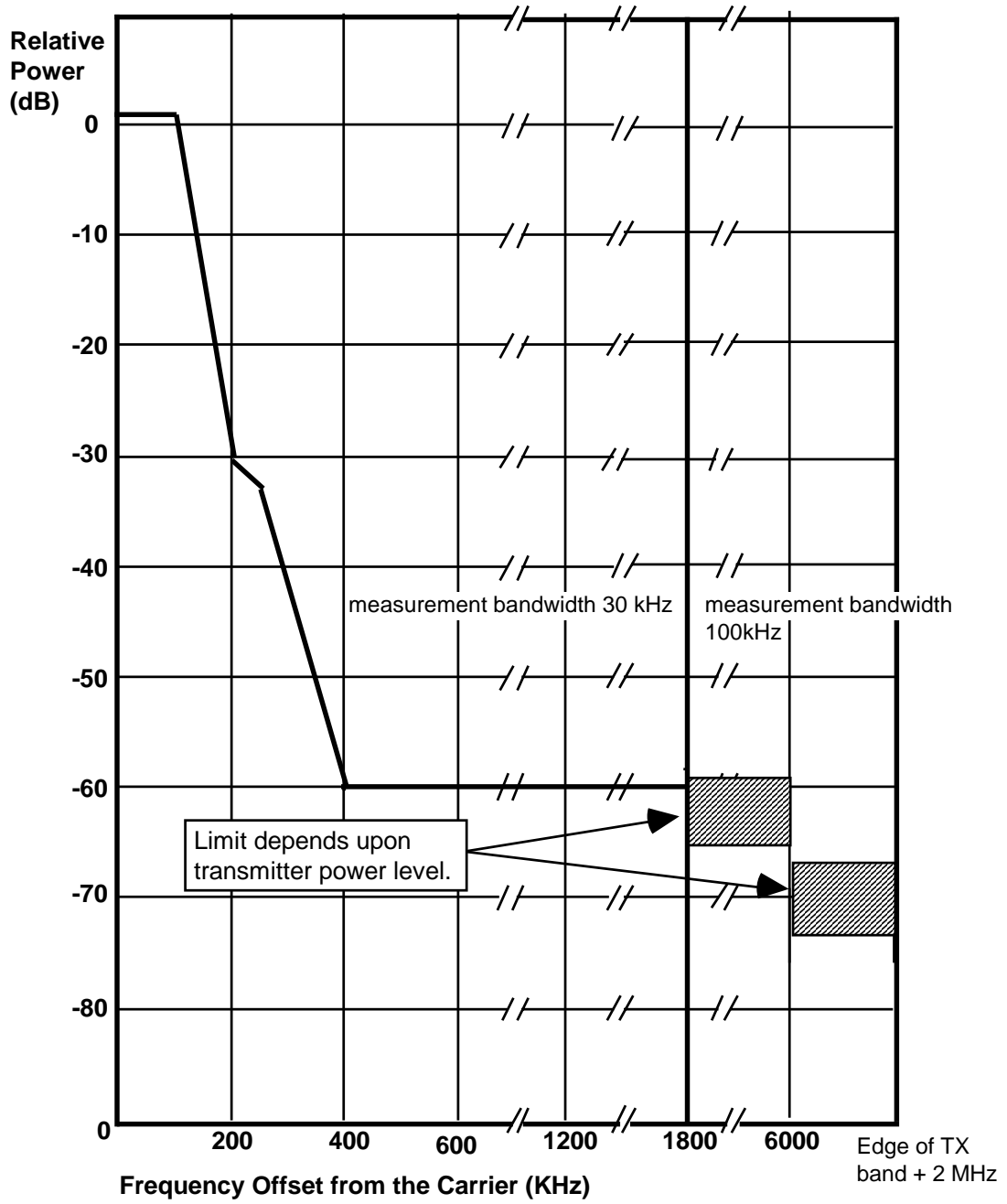
Figure A.5a: PCS 1 900 and MXM 1900 MS Modulation & Noise Spectrum Mask due to GMSK modulation
