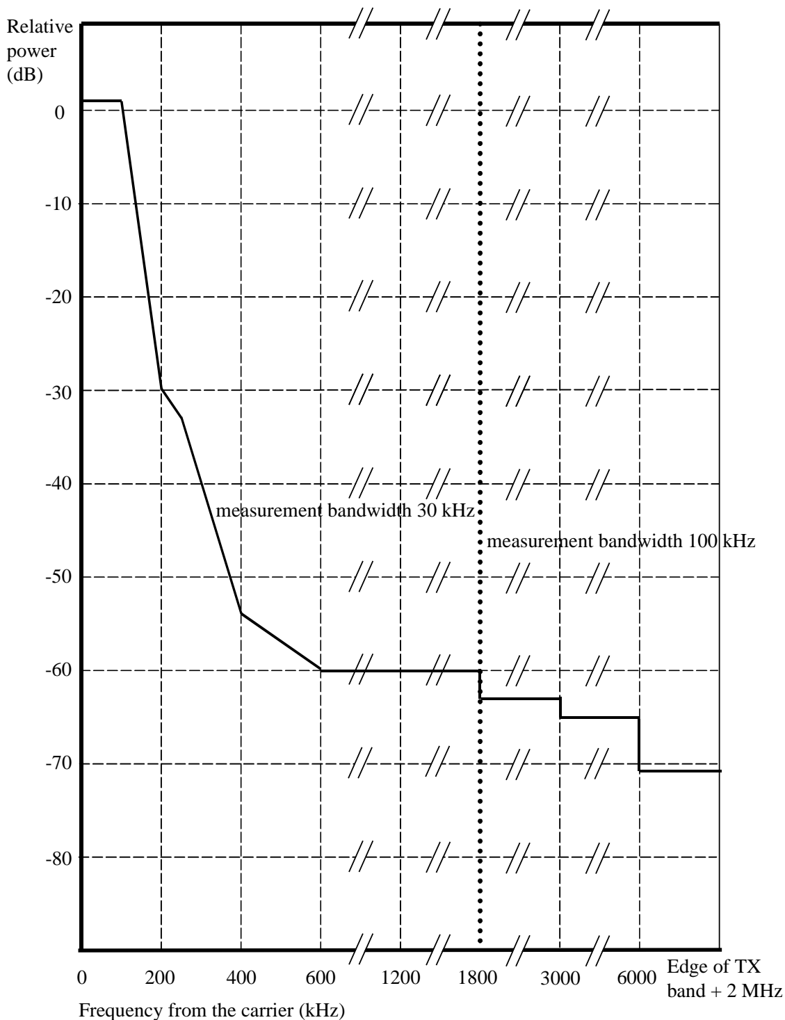
Figure A.1b: GSM 400 and GSM 900 and MXM 850 MS spectrum due to 8-PSK modulation
