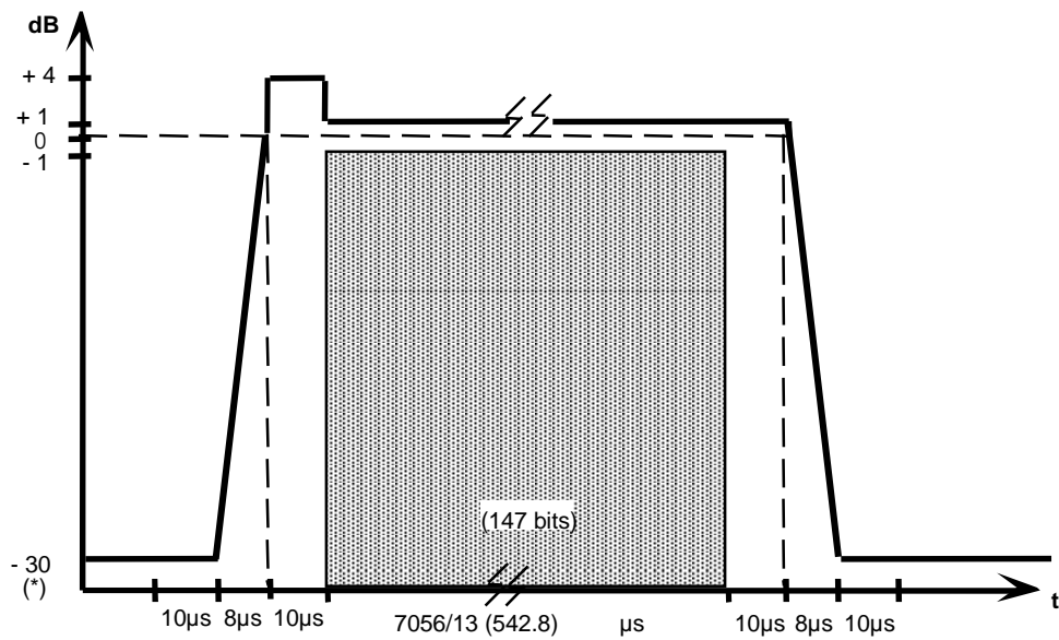
Time mask for access bursts (AB)
