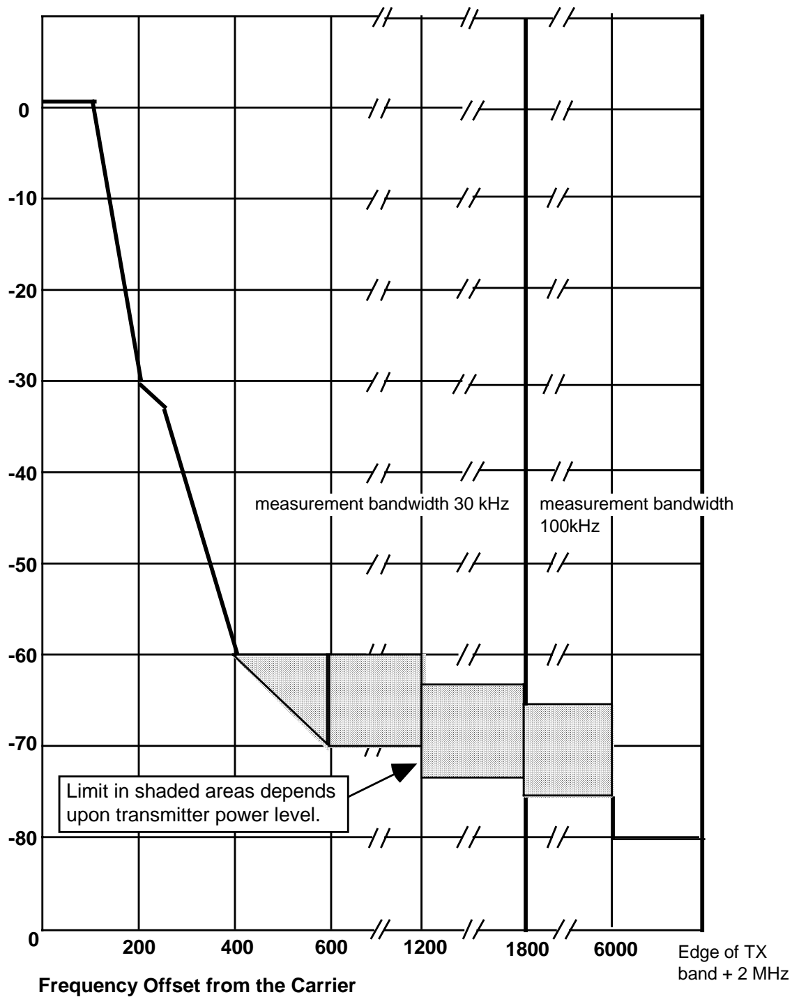
Figure A.6a: PCS 1 900 and MXM 1900 BTS Modulation & Noise Spectrum Mask due to GMSK modulation
