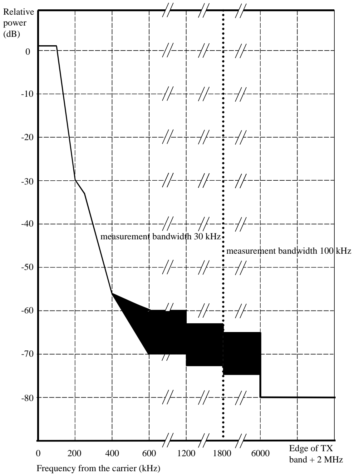
Figure A.2b: GSM 400 and GSM 900 and MXM 850 BTS spectrum due to 8-PSK modulation
