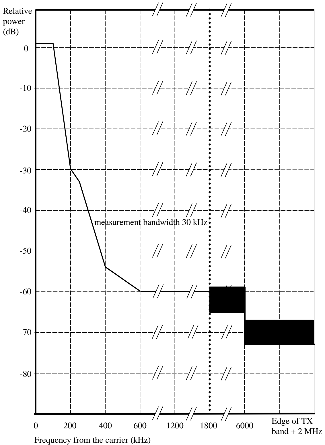
Figure A.5b PCS 1900 and MXM 1900 MS Modulation & Noise Spectrum Mask due to 8-PSK modulation
