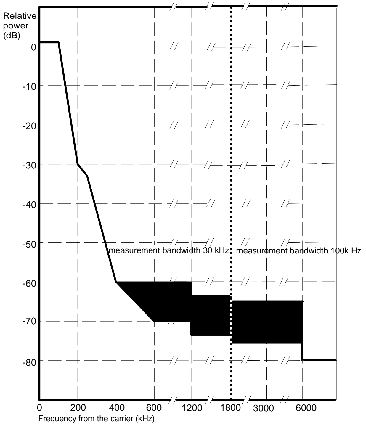
Figure A.2a: GSM 400, GSM 900 and MXM 850 BTS spectrum due to GMSK modulation
