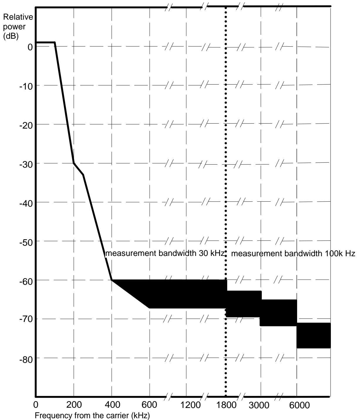
Figure A.1a: GSM 400, GSM 900 and MXM 850 MS spectrum due to GMSK modulation
