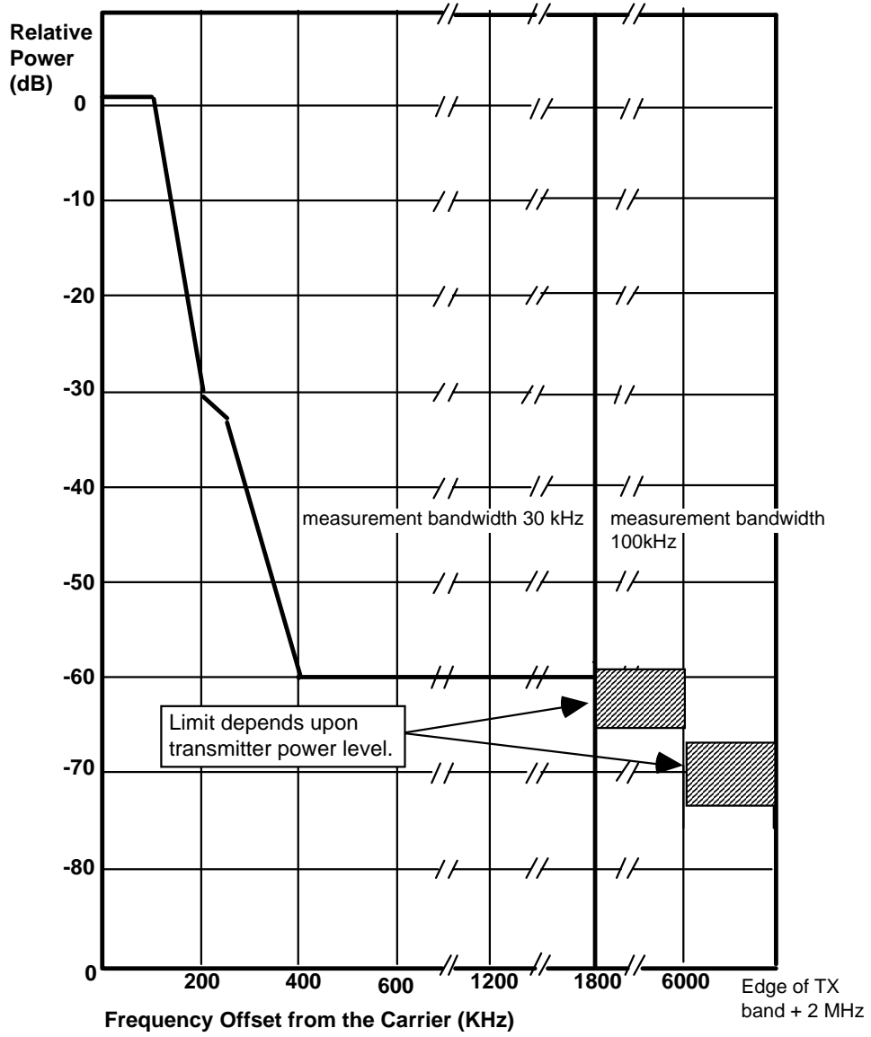
Figure A.5 PCS 1 900 MS Modulation & Noise Spectrum Mask
