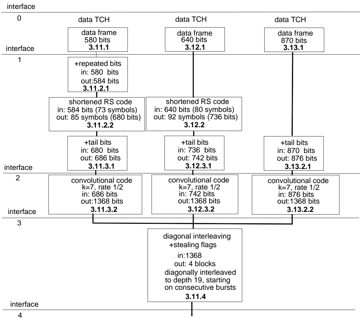
Figure 2a: Channel Coding and Interleaving Organization for ECSD 8-PSK modulated signals
