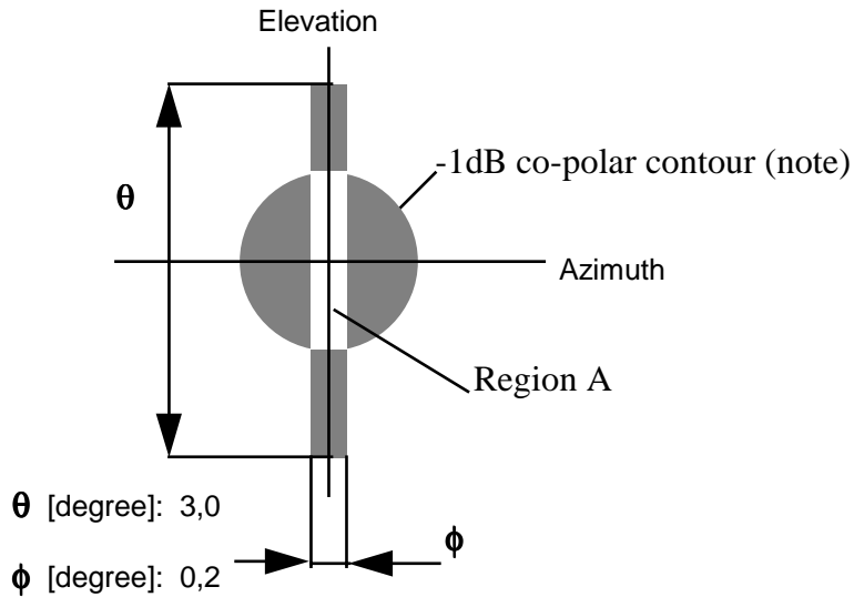
Figure 8: Mask for XPD measurements around the main beam axis
