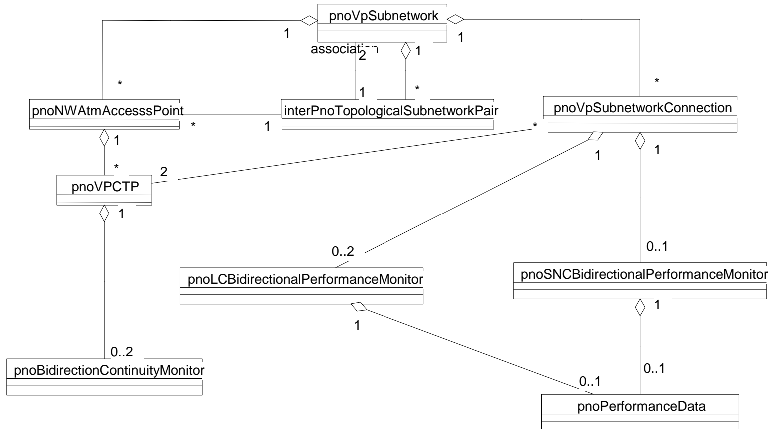
Figure 12: Entity Relationship diagram for PM object classes and CM object classes in UML notation
