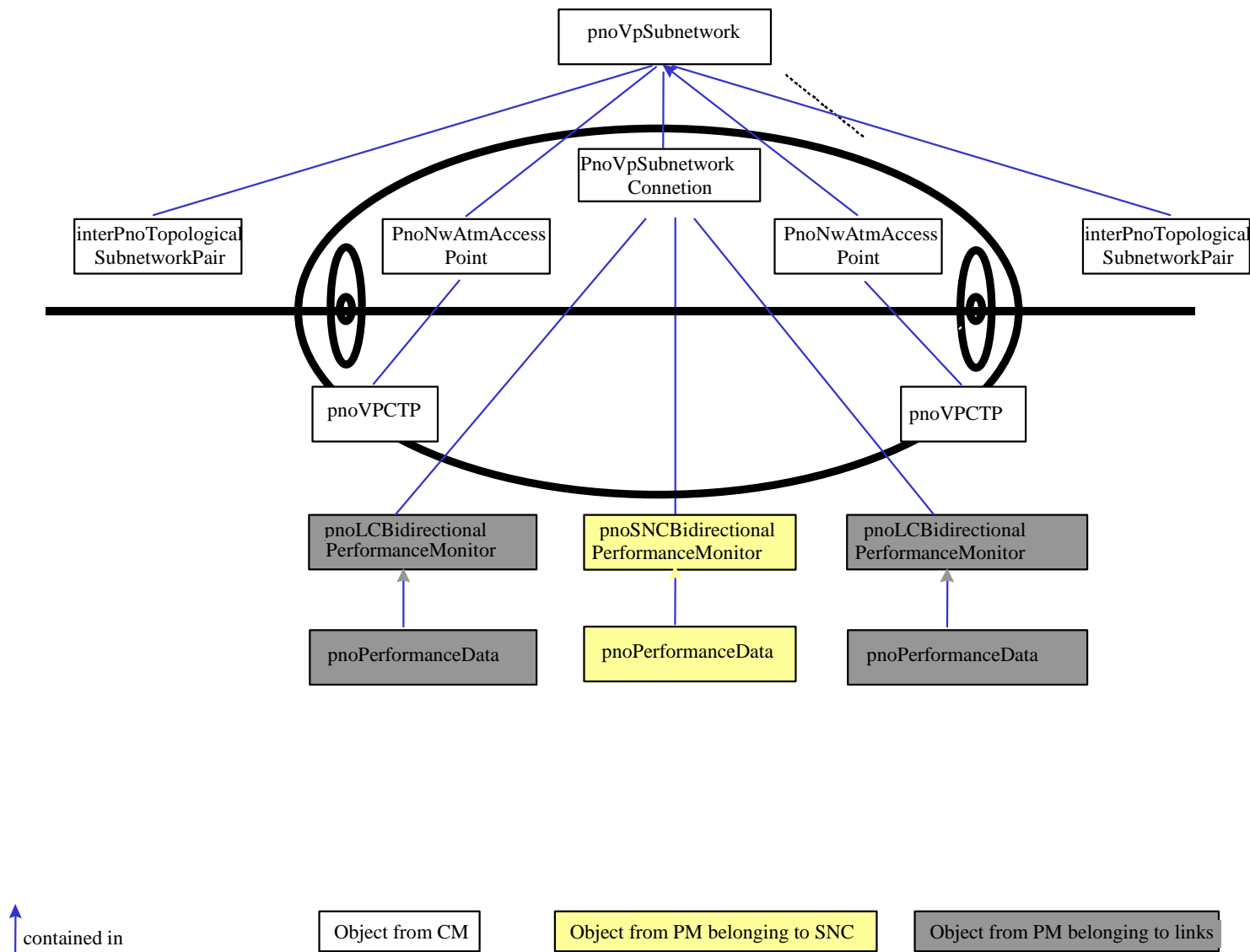
Figure 13: MIB for one Subnetwork
