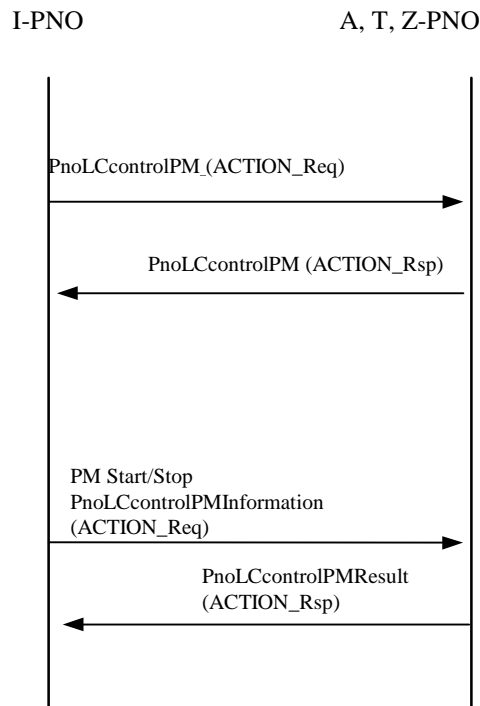
Figure 9: PM of a link connection
