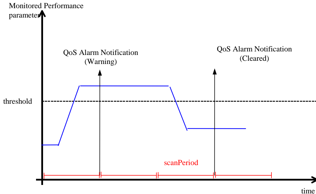
Figure 4: Occurrence of QoS Alarm and QoS Alarm Clearance Notification
