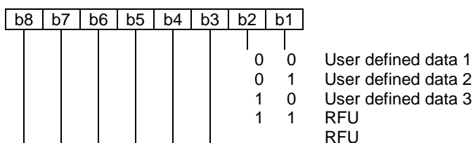
Figure 44: Message header
