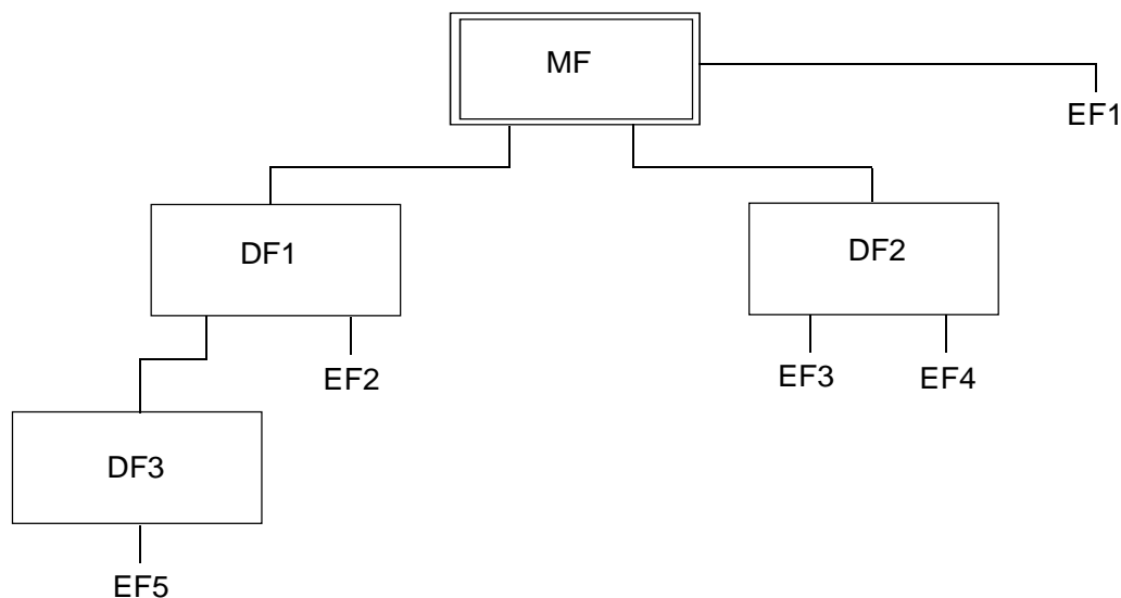
Figure 6: Logical structure
