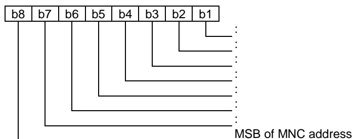
Figure 35: Network address
