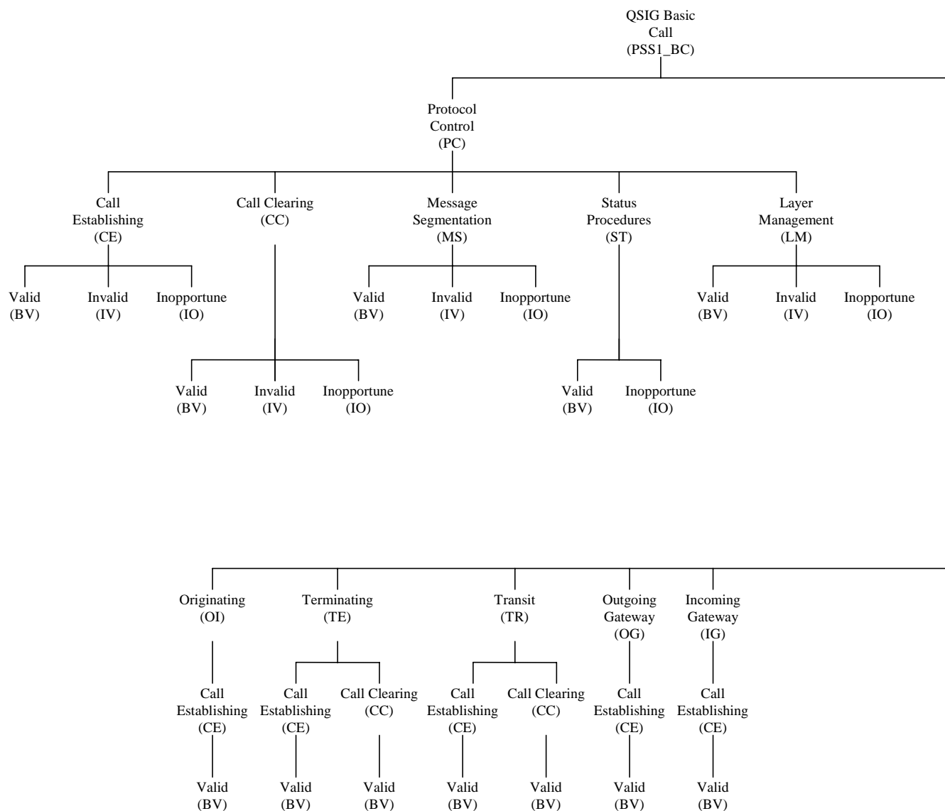
Figure 1: PSS1 Layer 3 Test Suite Structure overview
