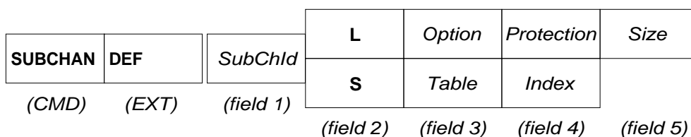
Figure 23: SUBCHAN DEF message structure
