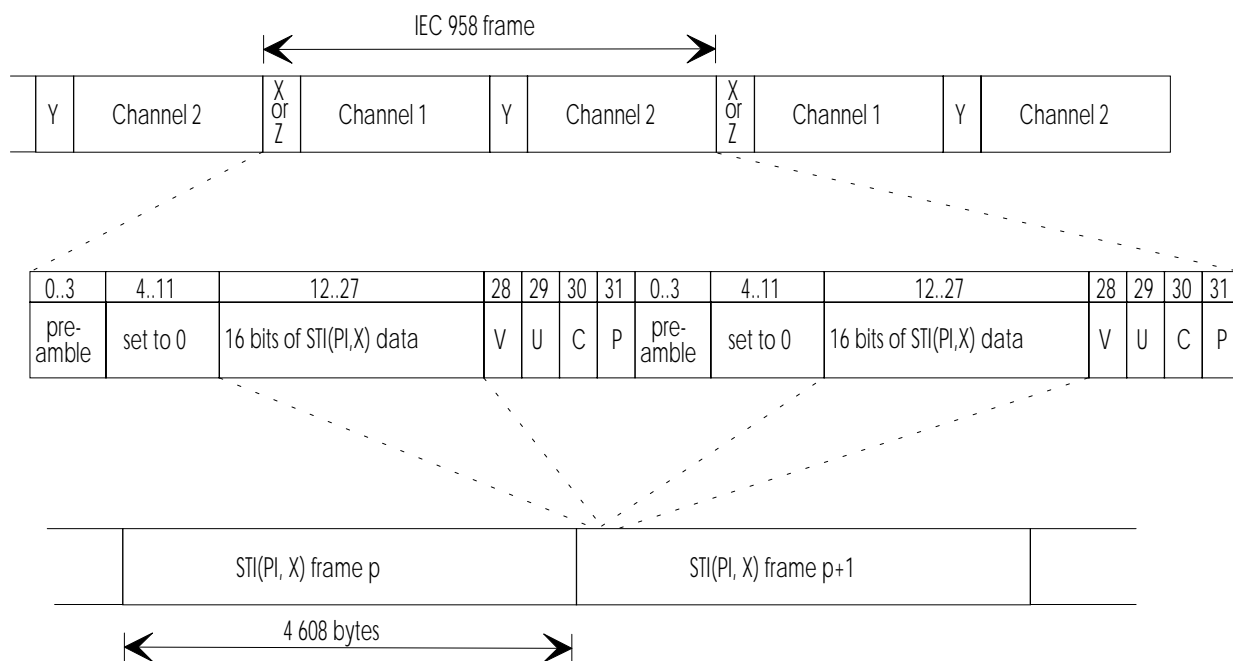
Figure 81: Physical adaptation of STI in the IEC958 frame
