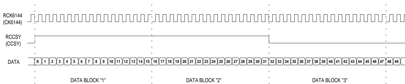
Figure C.2: Phase relationship of WG1/2 interface signals
