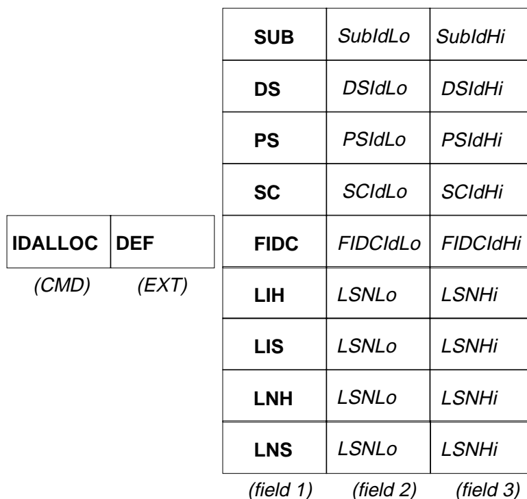
Figure 48: IDALLOC DEF message structure
