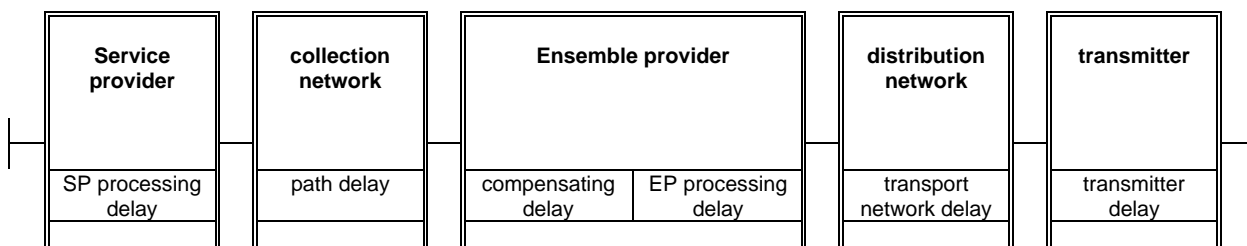
Figure F.2: Delay blocks in typical DAB network
