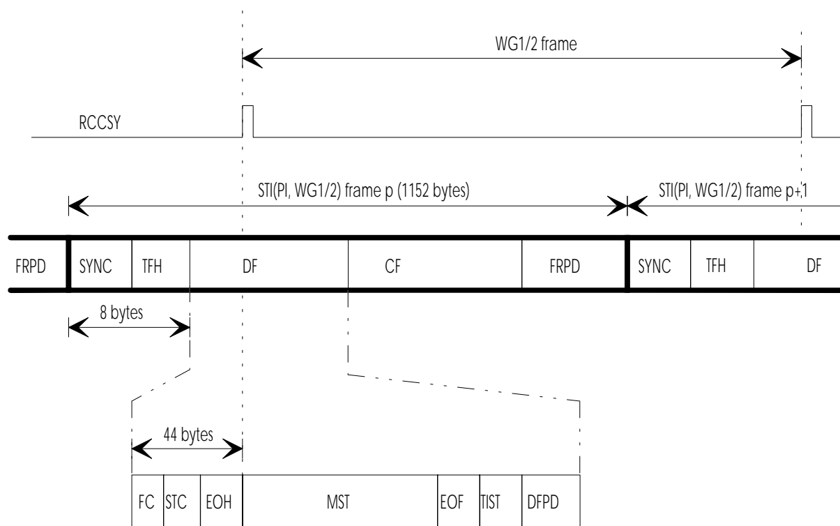
Figure 80: Adaptation of the STI(PI, WG1/2) frame to the WG1/2 frame
