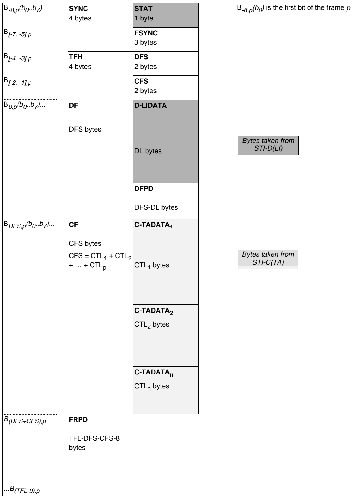
Figure 79: Mapping of STI-D(LI) and STI-C(TA) to the STI(PI, X)
