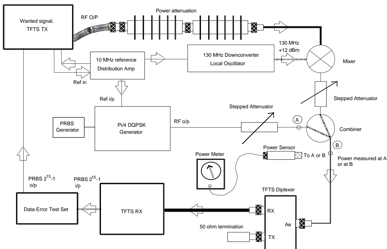
Figure 3: An example of a loopback facility for co-channel and adjacent channel measurements
