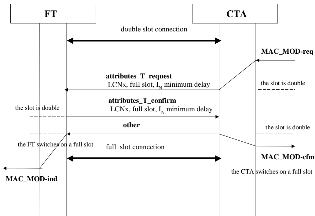
Figure 7: 64 kbit/s to 32 kbit/s switch, FT initiated
