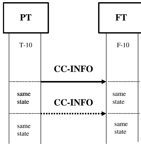
Figure 2: Sending on-hook/off hook information
