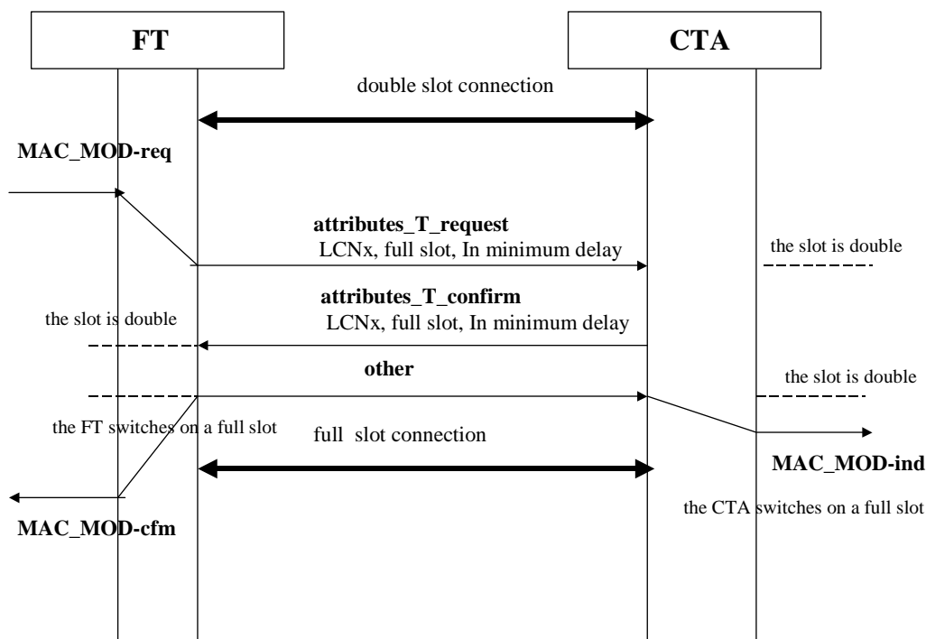
Figure 8: 64 to 32 kbit/s switch, CTA initiated
