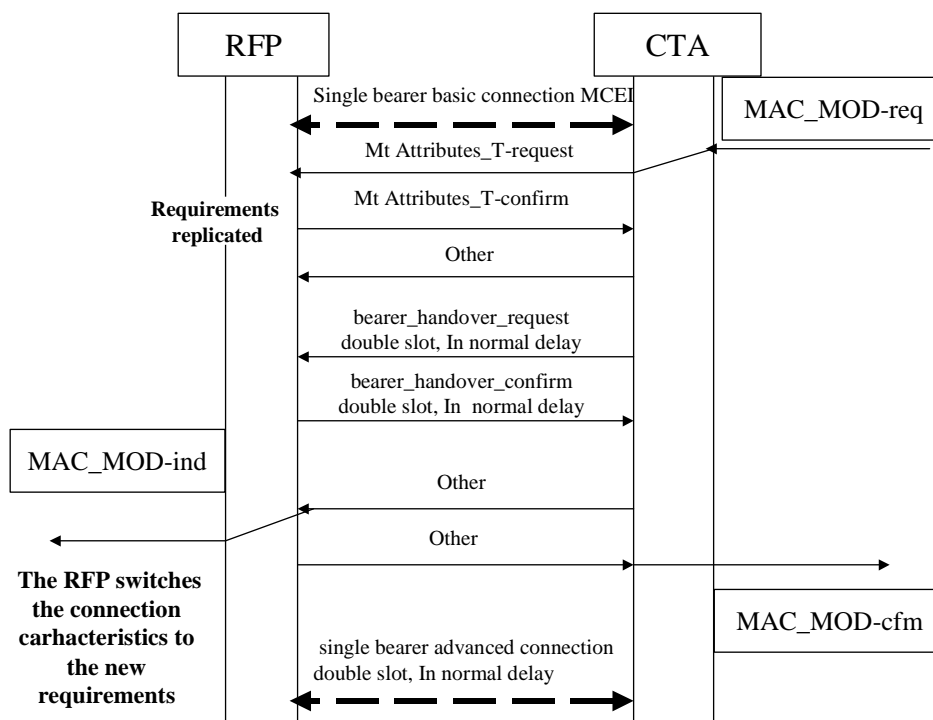
Figure 5: 32 to 64 kbit/s switch, FT initiated
