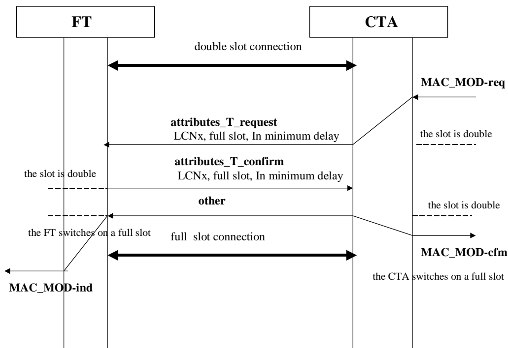
Figure 7: 64 to 32 kbit/s switch, FT initiated
