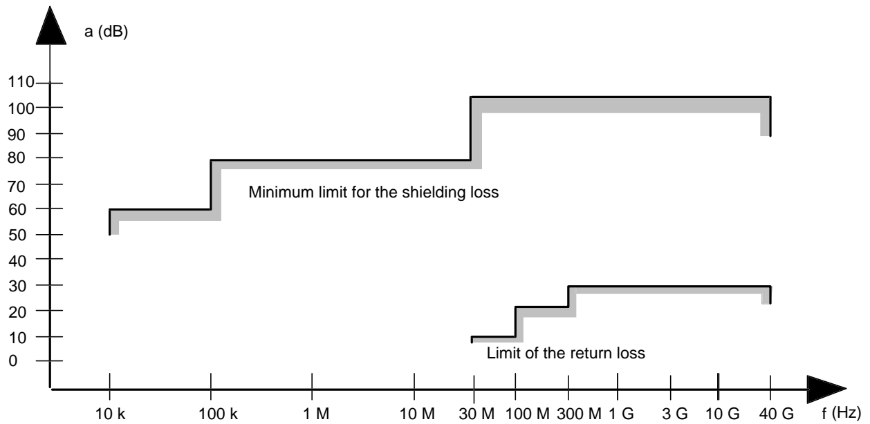
Figure A.3: Specification for shielding and reflections
