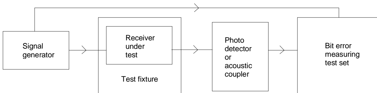
Figure 2: Measuring arrangement for calibration
