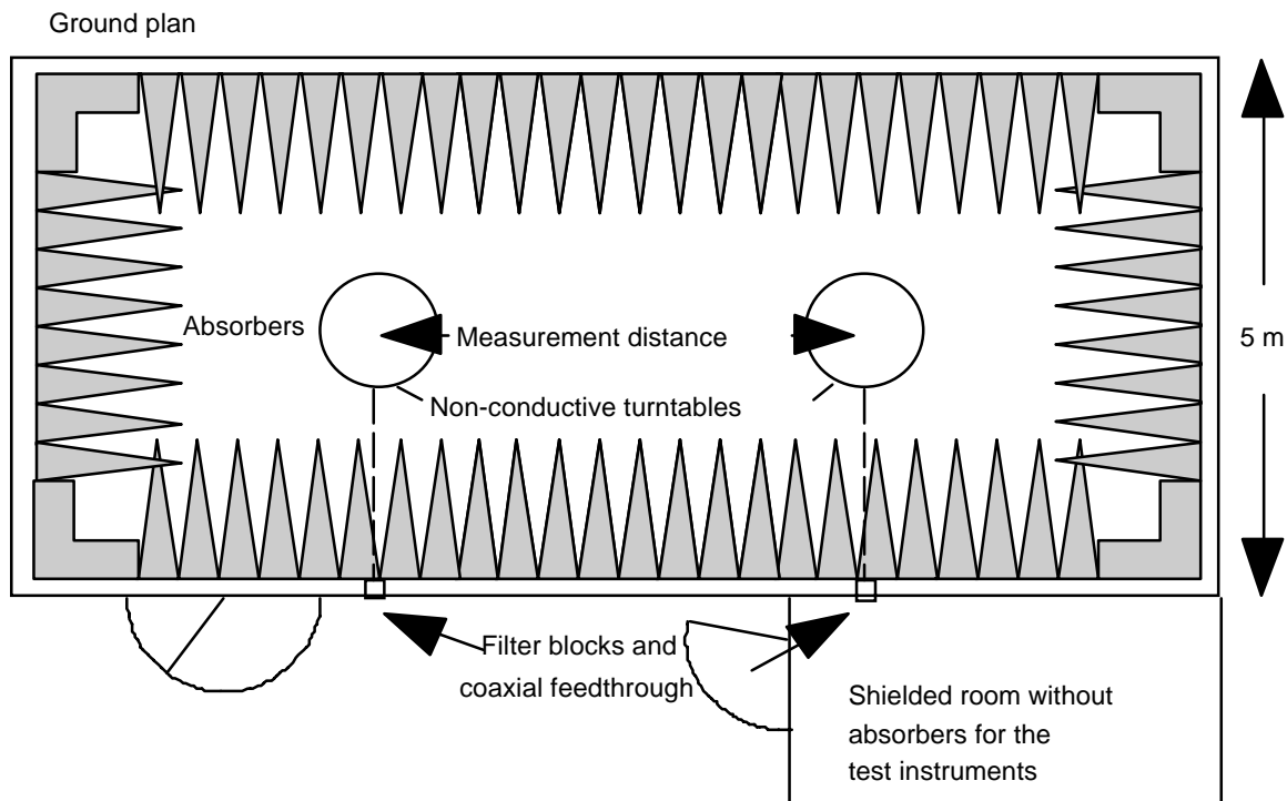
Figure A.4: Example of construction of an anechoic shielded chamber
