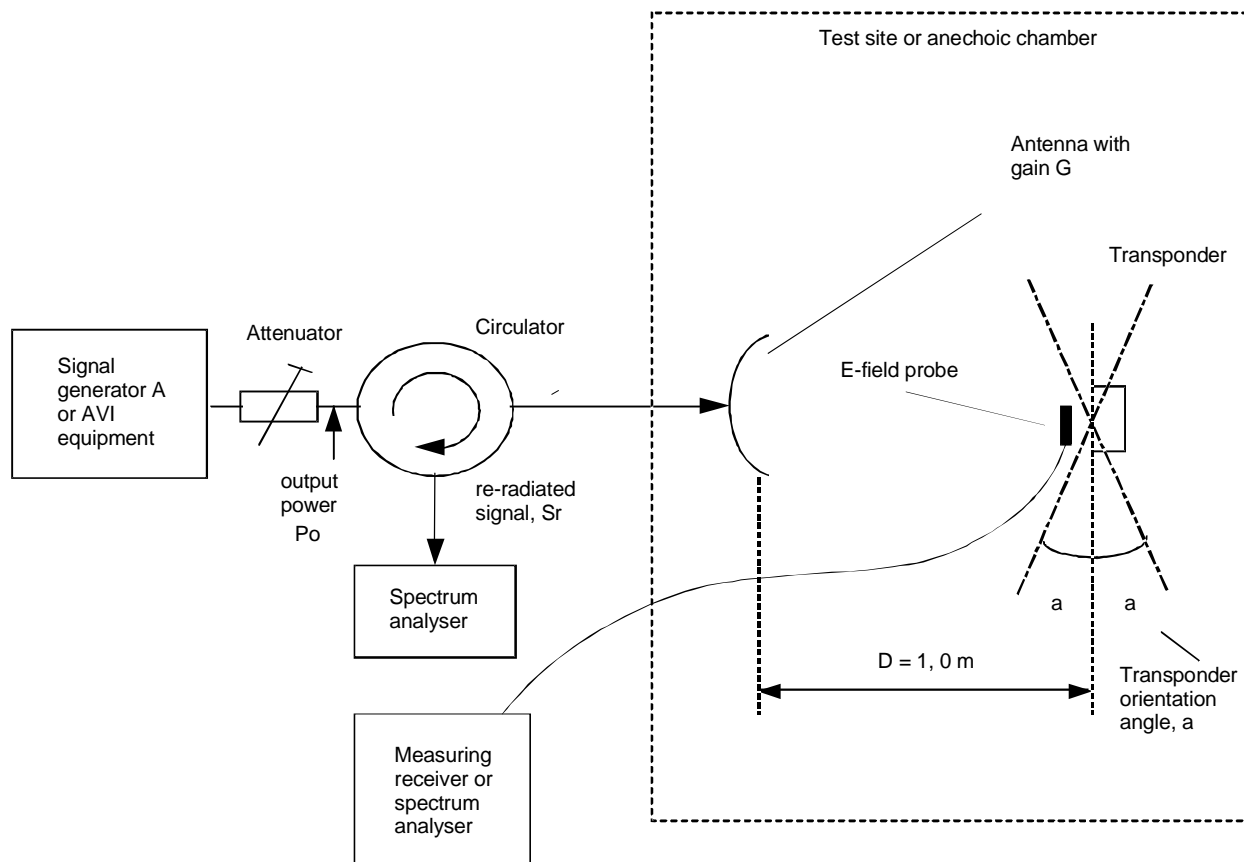
Figure 12: Test arrangement - transponder wake up
