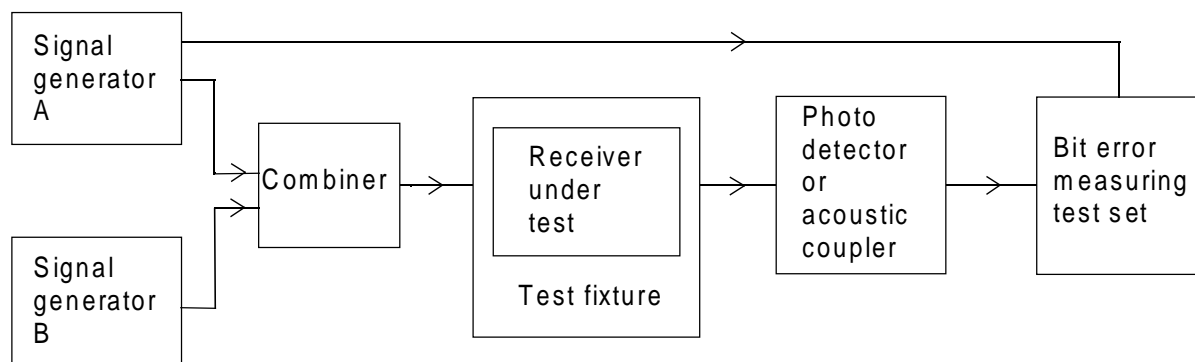
Figure 7: Measurement arrangement - co-channel rejection
