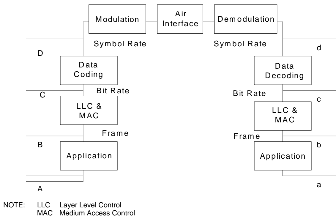
Figure 1: Measuring points for data stream measurements
