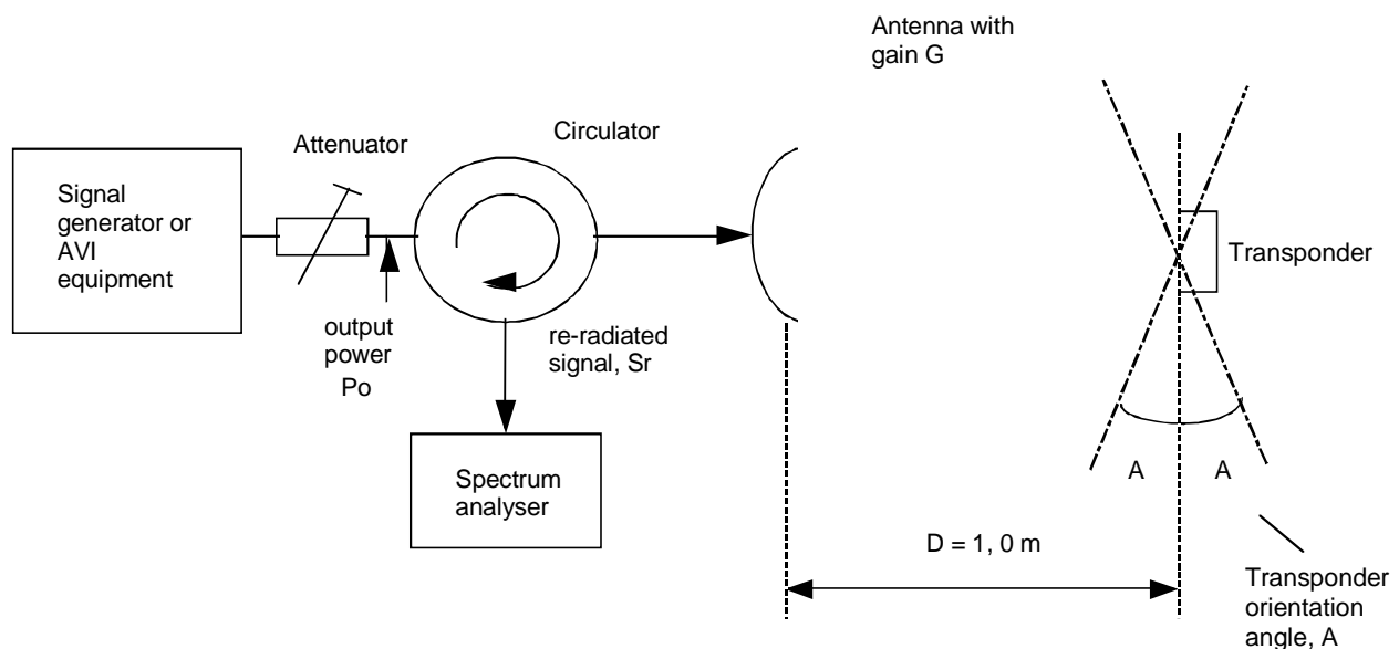
Figure 11: Measurement arrangement - transponder sensitivity
