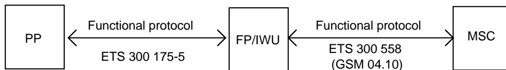
Figure 2: Transport mechanisms between DECT PP, FP/IWU, and GSM MSC
