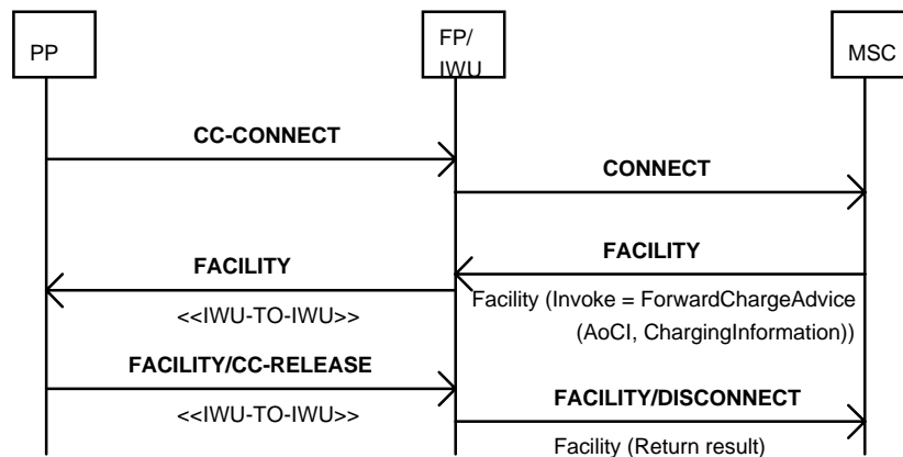
Figure 23: Message flow: notification to the served mobile subscriber of the charging information in case of a terminated call setup
