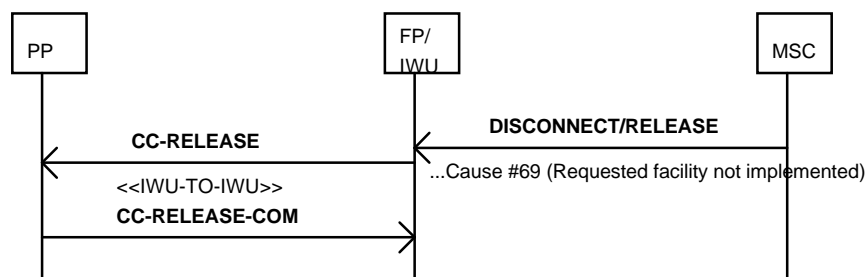
Figure 8: Message flow: Example for a network initiated release due to an unsuccessful operation (e.g. advice of charge (charging) service)
