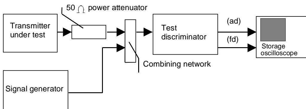
Figure 3: Measurement arrangement
