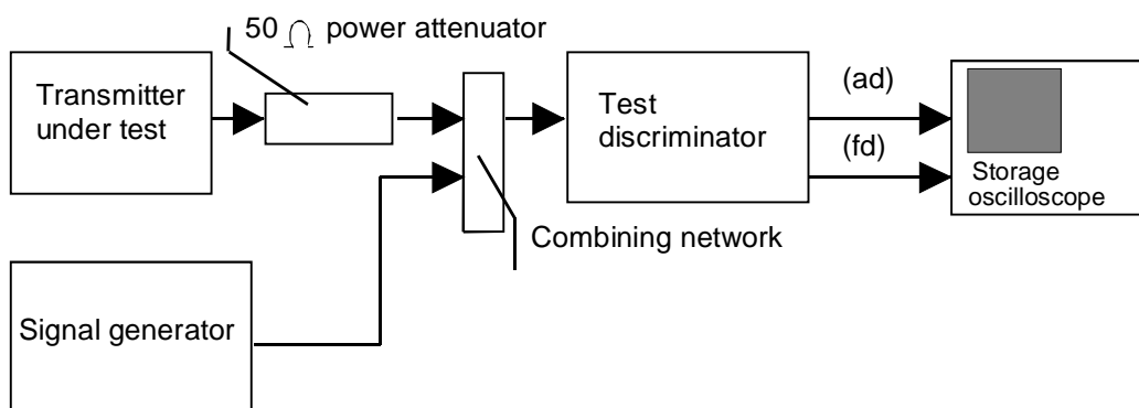
Figure 3: Measurement arrangement
