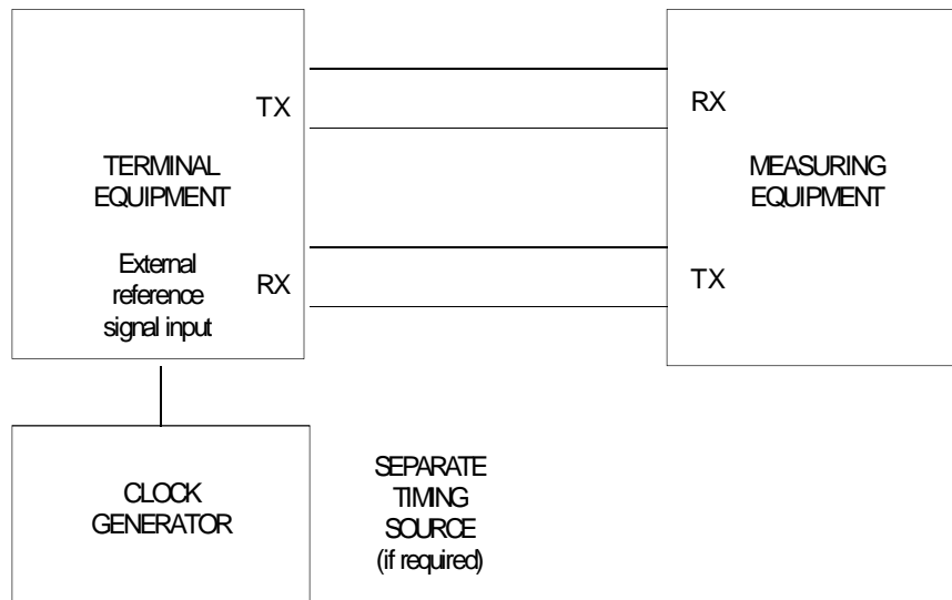
Figure A.3: Output timing
