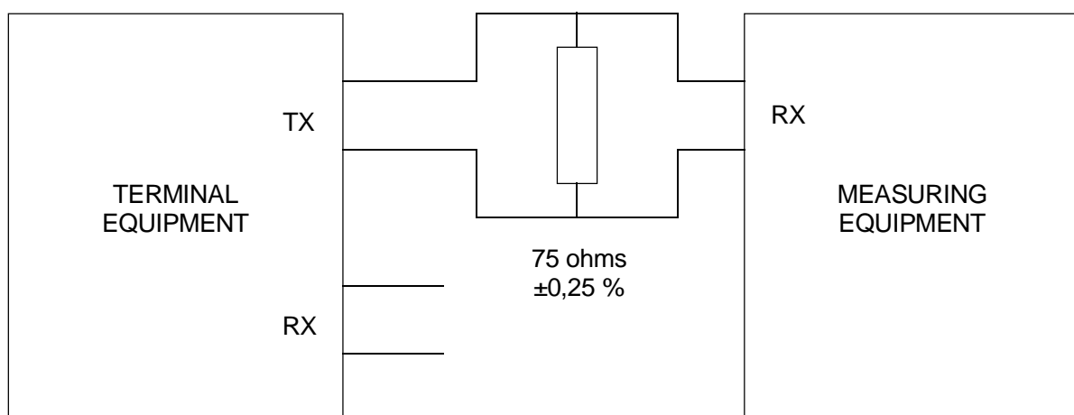
Figure A.2: Waveform shape at output port
