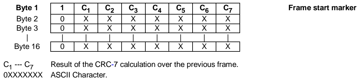
Figure C.3: 16-byte frame
