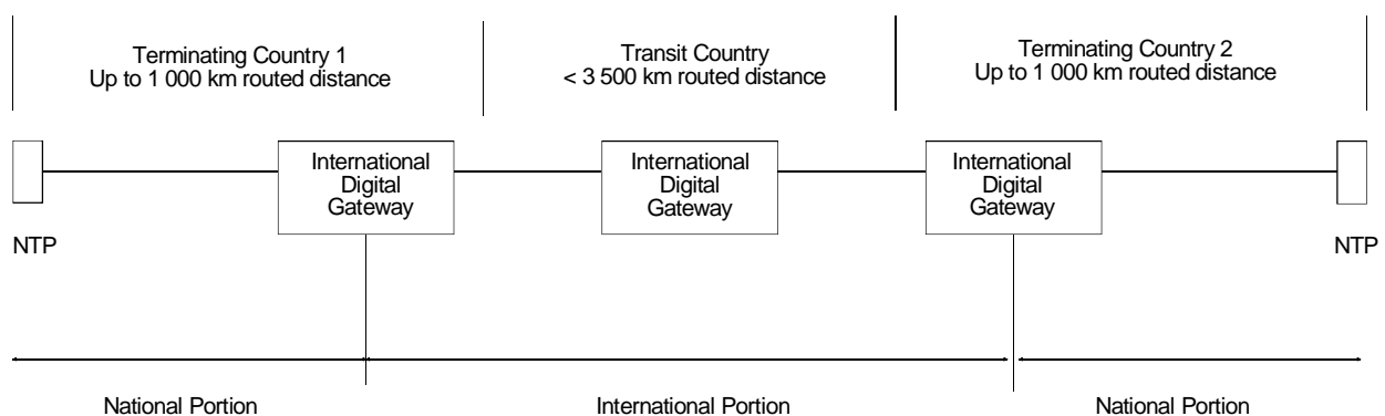
Figure C.1: Reference connection for terrestrial 34 Mbit/s digital leased line
