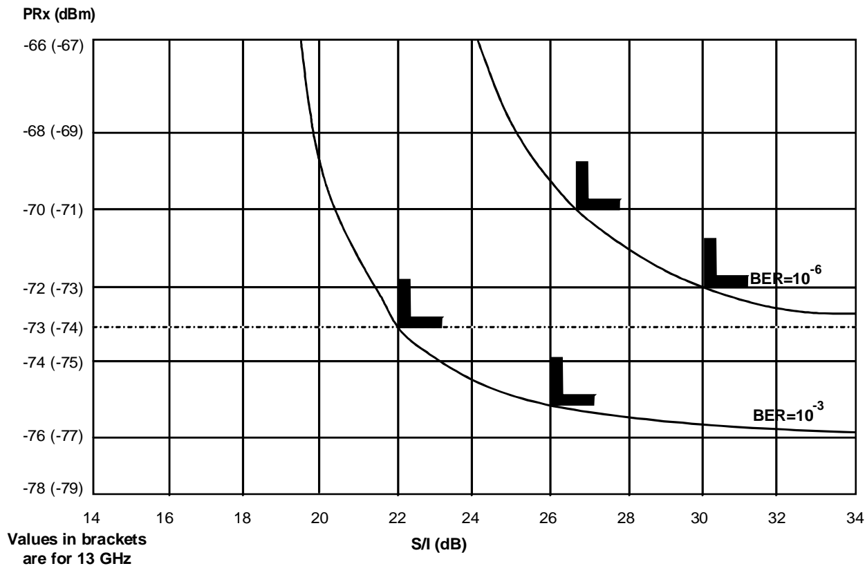
Figure 4: Co-channel digital interference mask for sub-STM-1, 13 GHz, 15 GHz and 18 GHz
