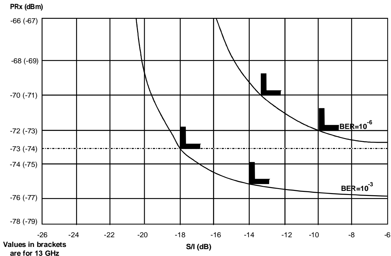
Figure 5: Adjacent channel digital interference mask for sub-STM-1,13 GHz, 15 GHz and 18 GHz (28/27,5 MHz channel spacing)
