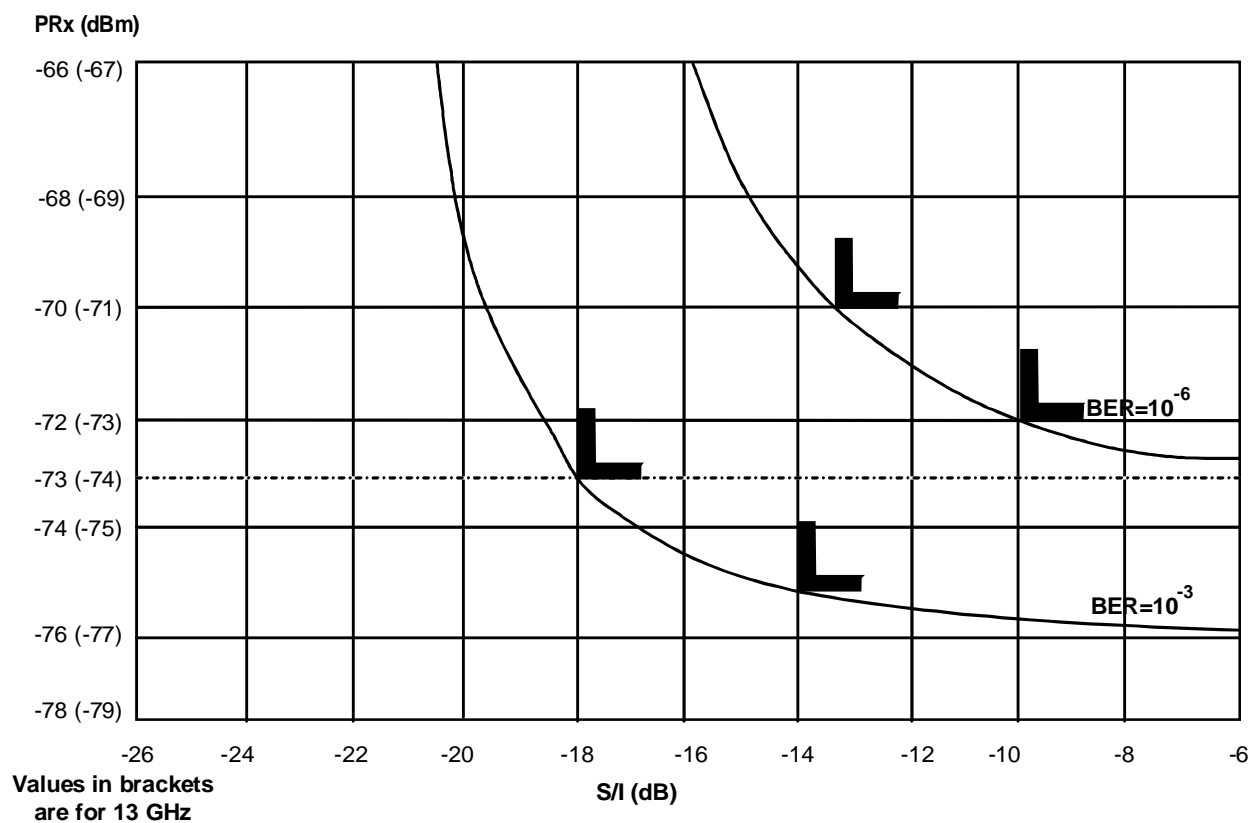
Figure 4: Adjacent channel digital interference mask for sub-STM-1, 13 GHz, 15 GHz and 18 GHz (28 / 27,5 MHz channel spacing)
