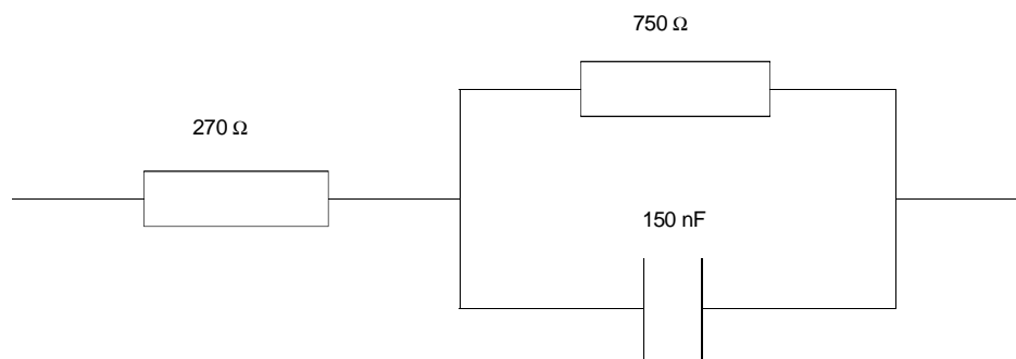
Figure A.1: Reference impedance Z_R
