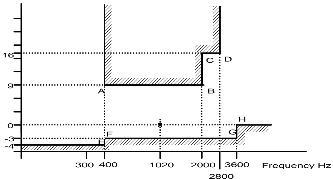
Figure 1: Limits for loss of the circuit relative to that at 1 020 Hz
