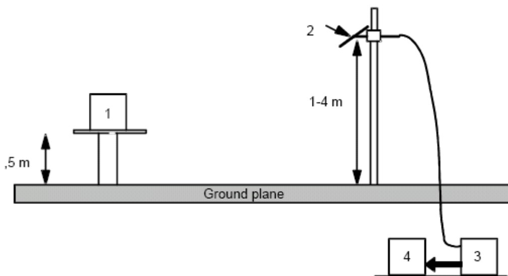
Figure A.1: Outdoor test site
