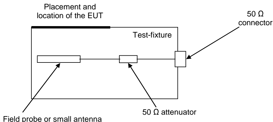
Figure 2: Test fixture
