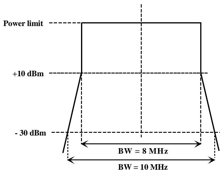
Figure C.1: Spectrum mask for RFID systems operating in the 2,45 GHz band
