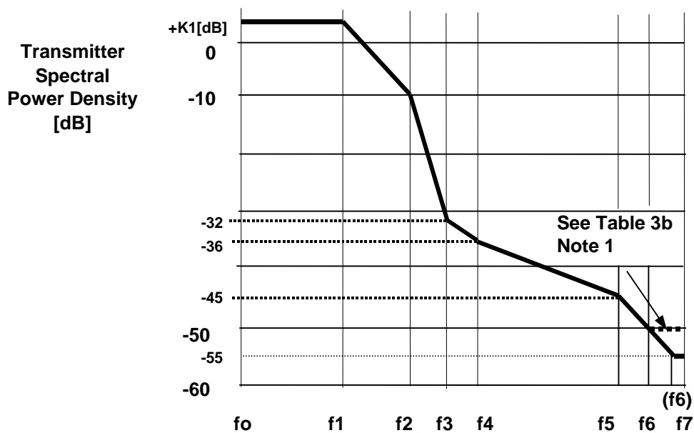
Figure 3b: Limits of spectral power density for Class 5a systems
