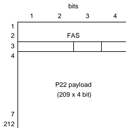
Figure 62: Decoded E22/P22e_AI_D signal
