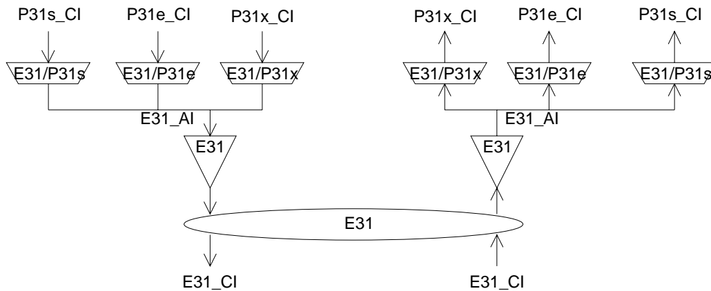
Figure 49: E31 Section atomic functions
