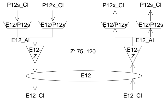
Figure 69: E12 Section atomic functions
