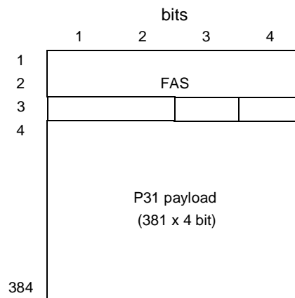
Figure 50: Decoded E31/P31e_AI_D signal
