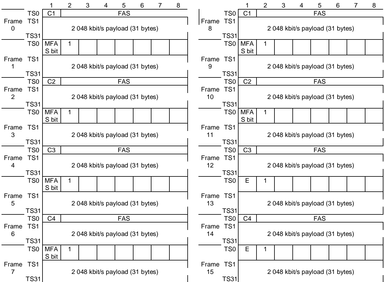
Figure 71: Decoded P12s_CI_D (with CRC-4 multiframe)
