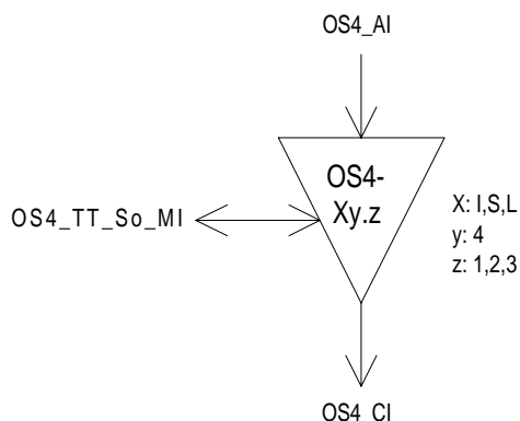
Figure 11: OS4-Xy.z_TT_So symbol
