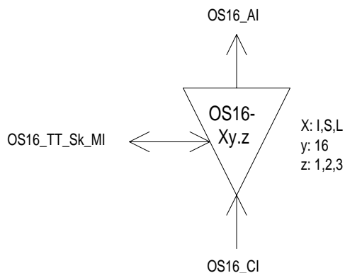
Figure 20: OS16-Xy.z_TT_Sk symbol
