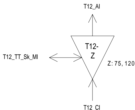
Figure 76: T12-Z_TT_Sk symbol
