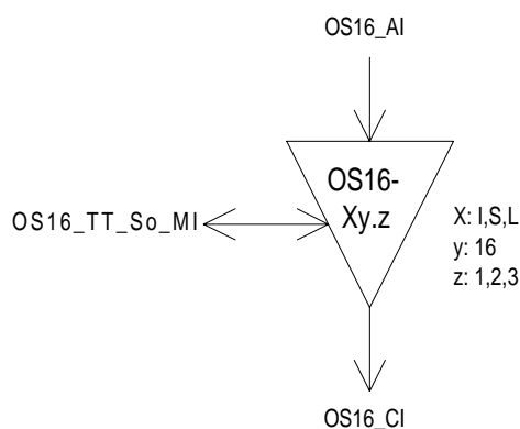
Figure 19: OS16-Xy.z_TT_So symbol
