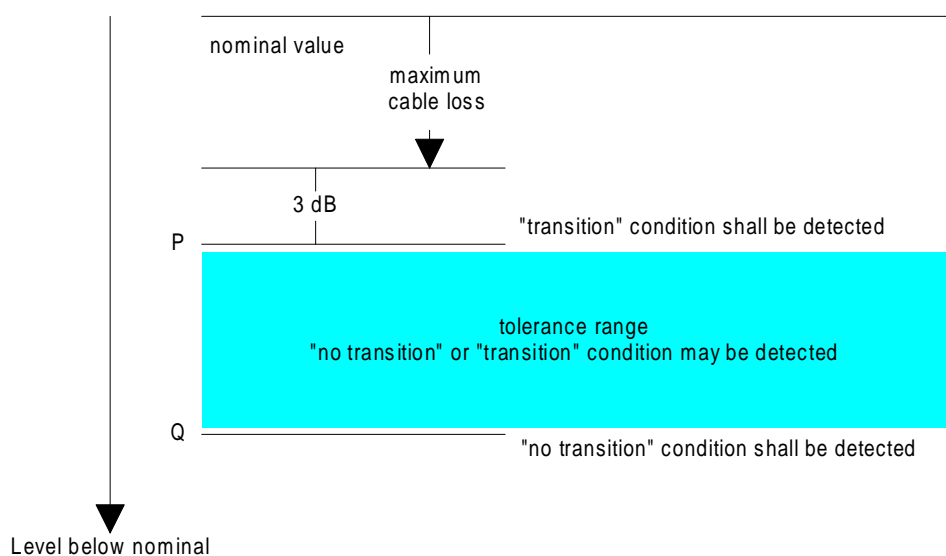
Figure 41: Criteria for determination of transition conditions
