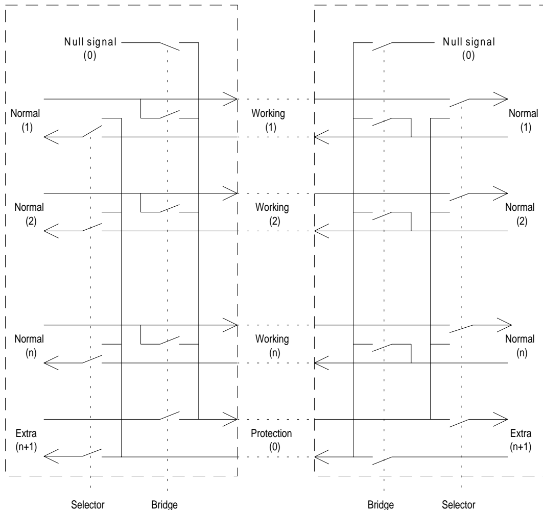
Figure 47: 1:n protection architecture
