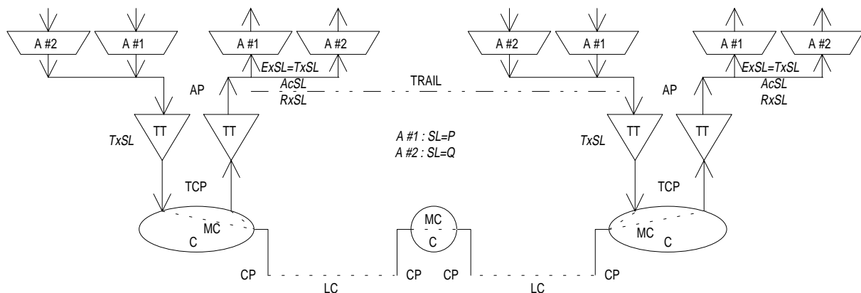
Figure 26: A bi-directional trail and its Signal Label parameters
