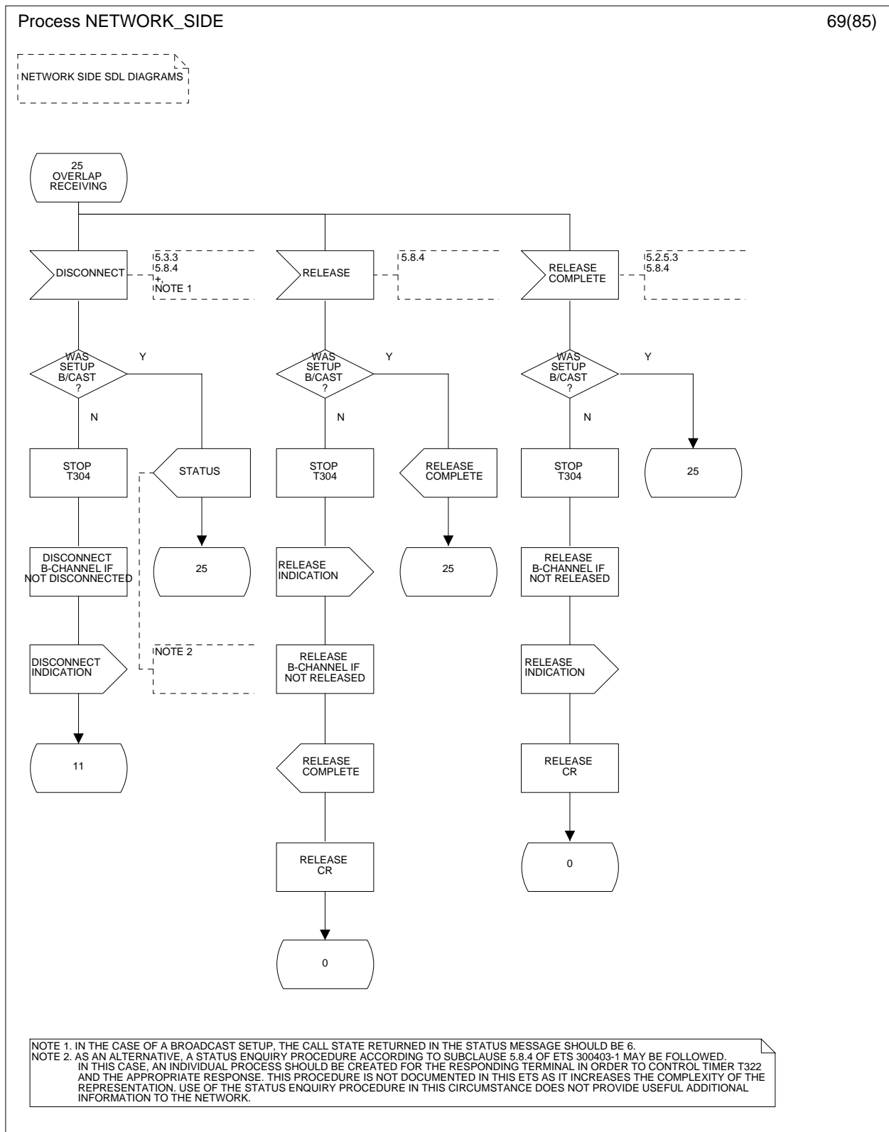
Figure 5 (sheet 69 of 85): Network side SDL diagram
