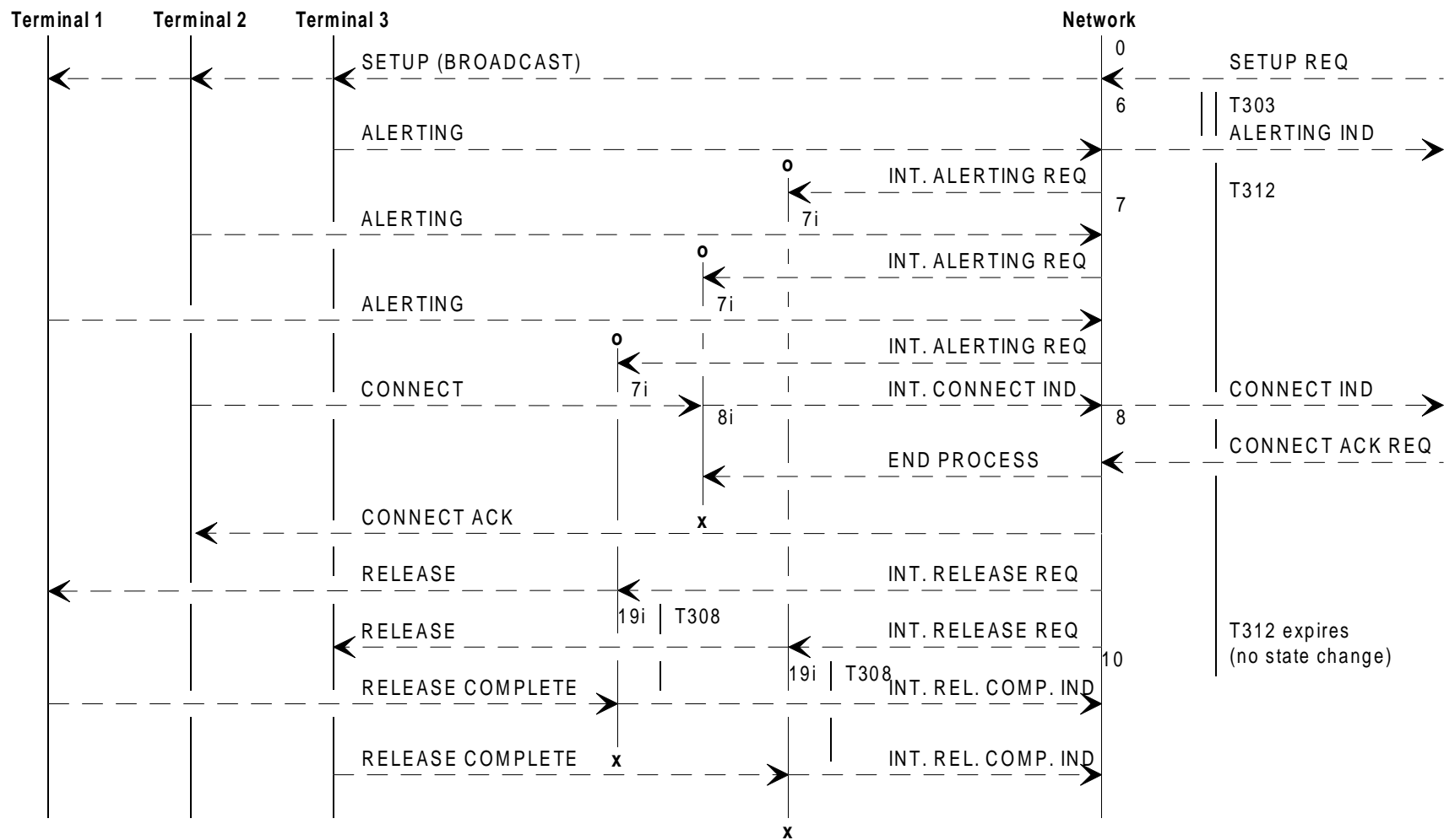
Figure 2: Multipoint call establishment (and clearing of non-selected terminals)
