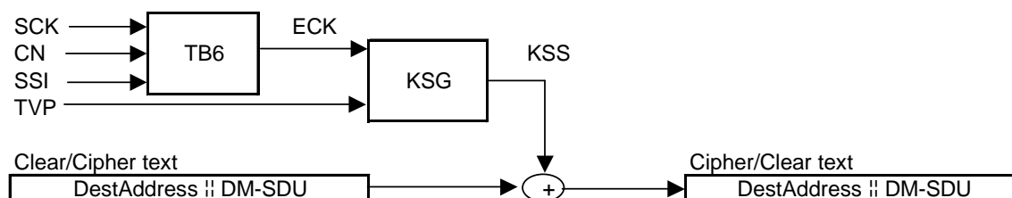
Figure 6: Encryption process as it occurs in TETRA DMO Class DM-2-B
