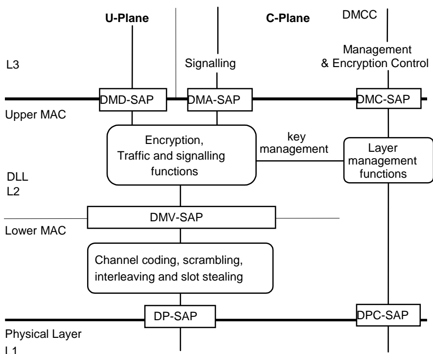
Figure 3: Relationship of security functions to layer functions
